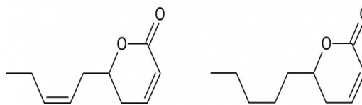
Tuberolactone
