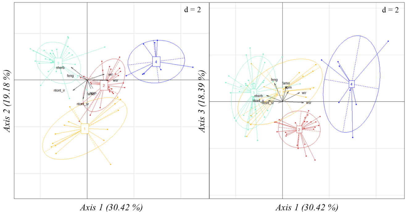
Figure 11: Graphs of the 4 groups displayed after a PCA applied on the 101 plots in function of the practices (black arrows)
