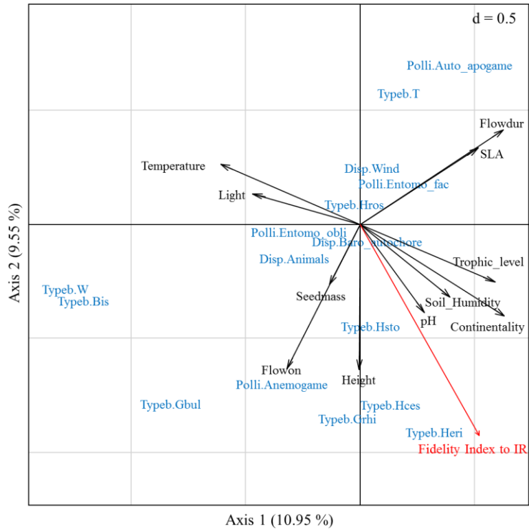
Figure 3: Hill & Smith analysis displayed with the quantitative variables in black marked out by an arrow, the qualitative variables in blue and the supplementary variable: Fidelity Index in the inter-rows in red marked out by an arrow.
