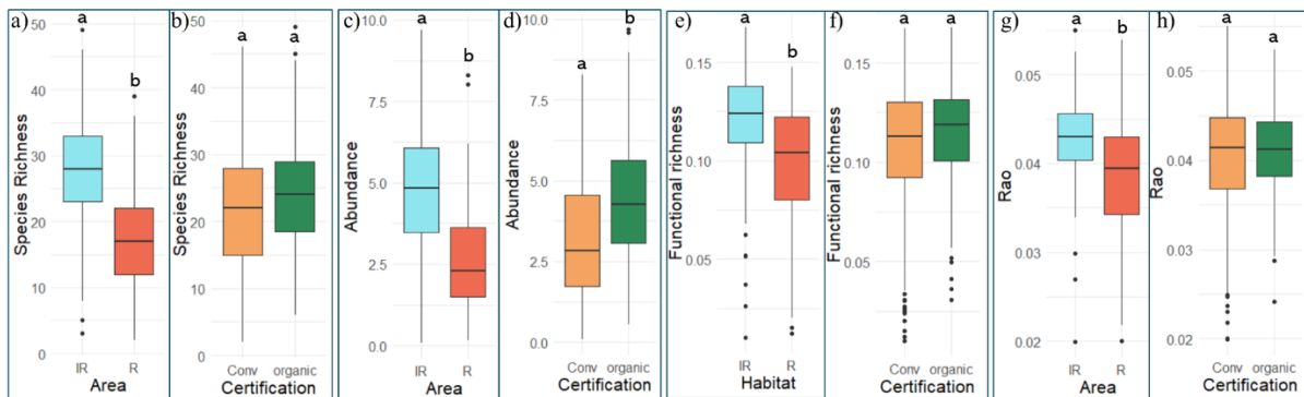
Figure 5: Diversity's indices, i.e. the species richness (a,b), the abundance (c,d), the functional richness (e,f) and the Rao's quadratic entropy (g,h), according to the area (inter-rows in blue, rows in red), the mode of production called here certification (conventional in orange and organic in green). The horizontal bar of the boxplot represents the median, 50% of the values were located from the 1 st quartile to the 3 rd quartile (interquartile range, IQR). Black dots are values higher or lower than 1.5 the IQR.
