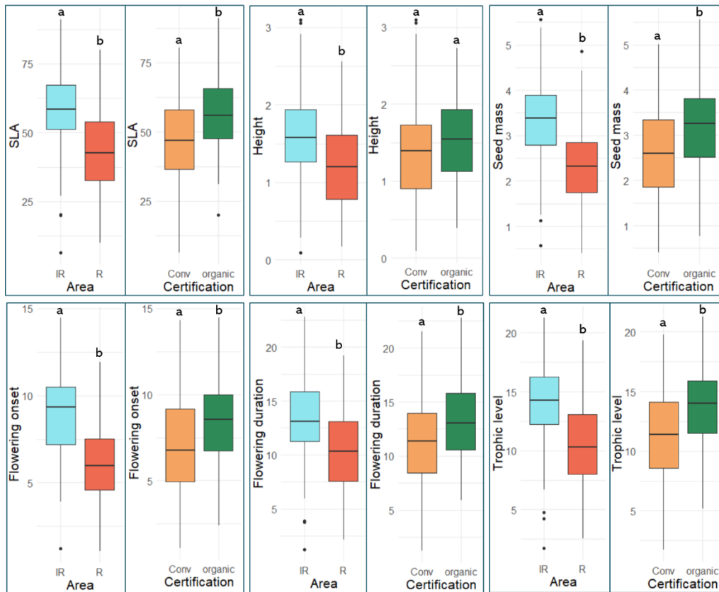
Figure 14: Boxplots of CWV of traits with the areas in blue for the inter-rows, in red for the rows, in yellow for conventional and in green for organic production mode.
