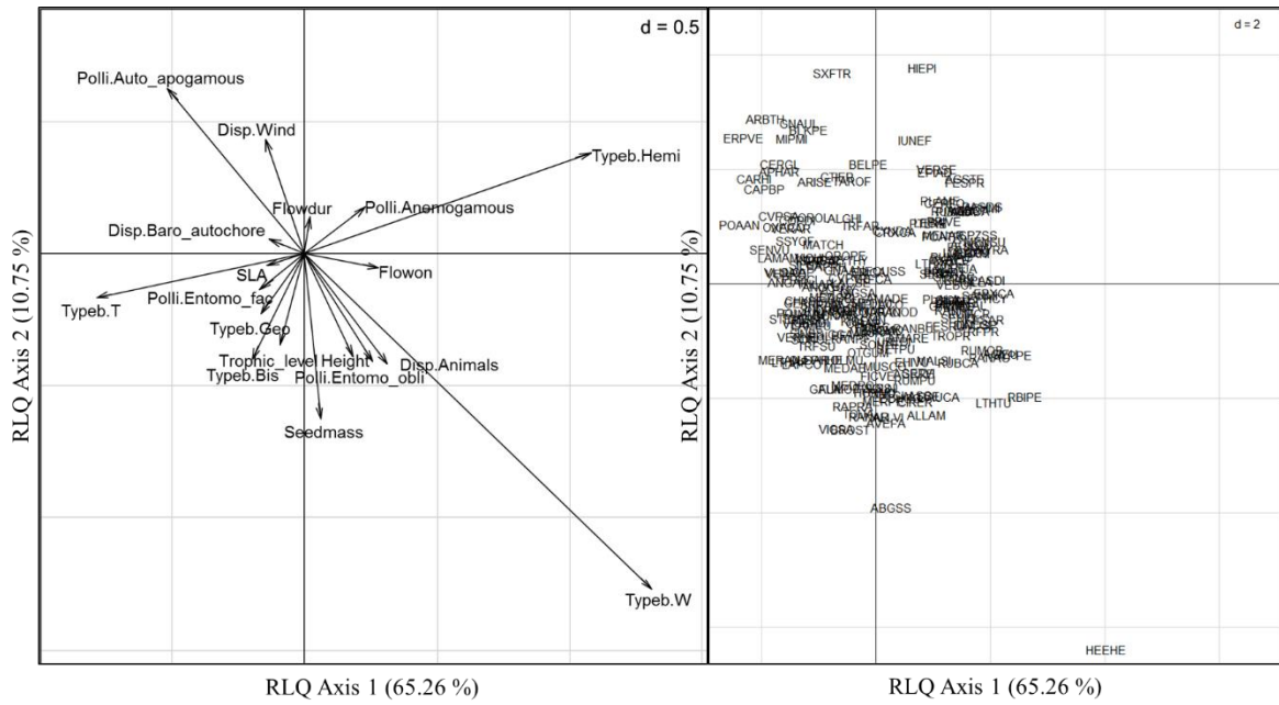
Figure 7: Results of the global RLQ (101 fields) for the traits (on the left) and the species (on the right)
