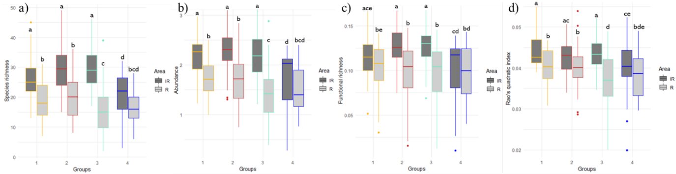
Figure 6: Boxplots of the repartition of the four groups depending on the diversity's indices: Species richness (a), Abundance (b), Functional richness (c) and Rao's quadratic entropy (d). The inter-rows were represented in dark grey and the rows in pale grey, the group 1 is in yellow, the group 2 in red, the group 3 in green and the group 4 in blue.
