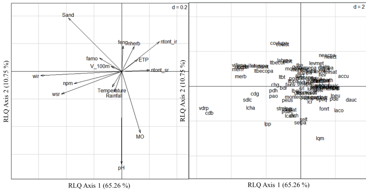
Figure 8: Results of the global RLQ (101 fields) for the environment variables (on the left) and the field (on the right)
