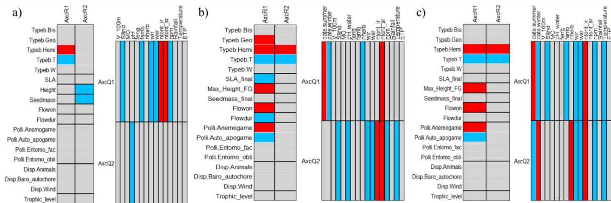
Figure 10: Results of the combination of the RLQ and the fourth-corner analyses for the global (a), the rows (b) and the inter-rows (c) analyses. On the left of each table, the fourth-corner tests between the two axes of the RLQ for the environmental gradients and the practices (AxcR1/AxcR2) and traits. On the right of each table, fourth-corner tests between the two axes of RLQ for traits (AxcQ1/AxcQ2) and the environmental variables and the practices.
