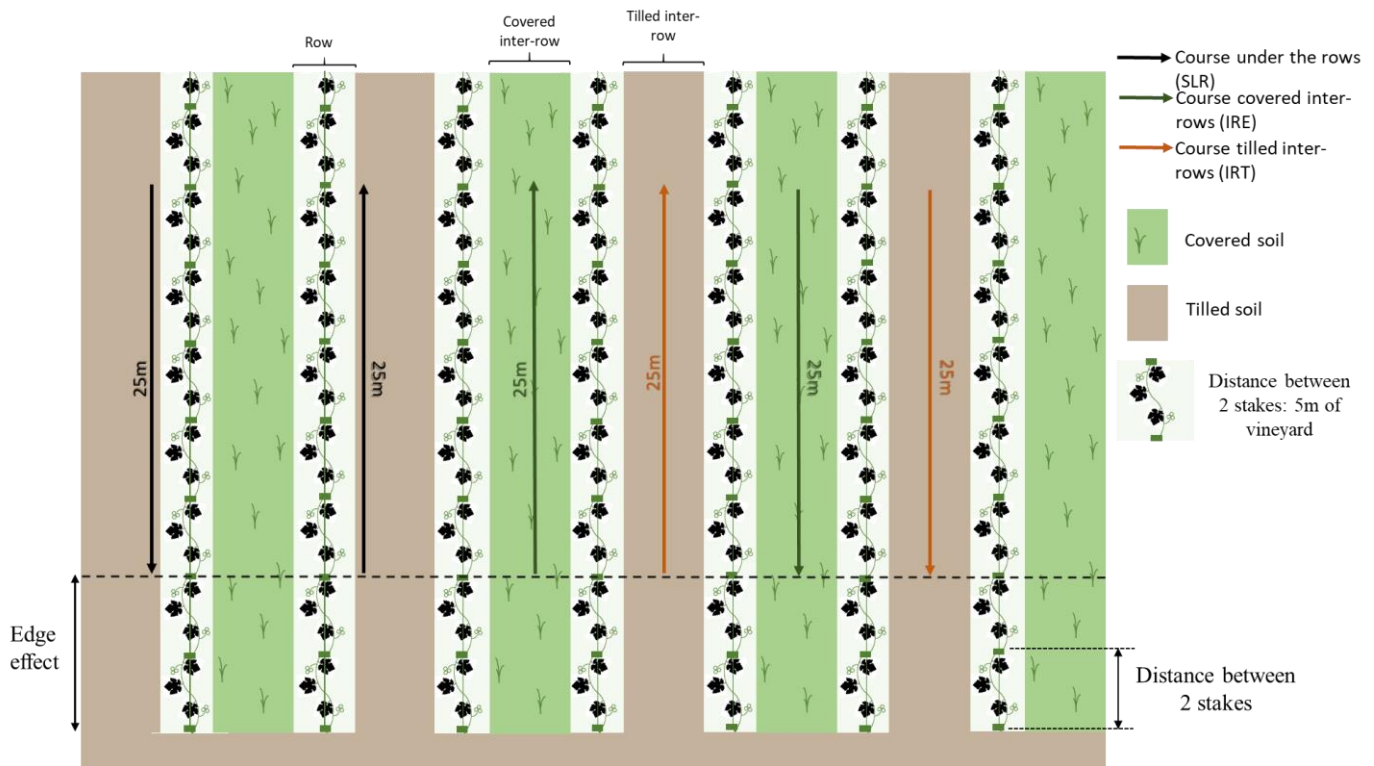
Figure 2: Scheme describing the method to provide the floristic sampling of each plot (took back from Varela (2015))
