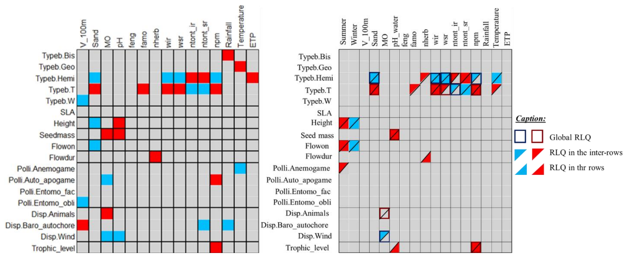
Figure 9: Fourth corner analysis of the global dataset (101 fields) on the left and adjusted fourth corner analyses of the three datasets (global, rows, inter-rows) on the right. The red cells represented the positive associations and the blue cells represented the negative associations. The non-significant cells were represented in grey. The upper left triangles represent the inter-rows significant interaction, the bottom right triangles the rows and the empty squares the global interaction.
