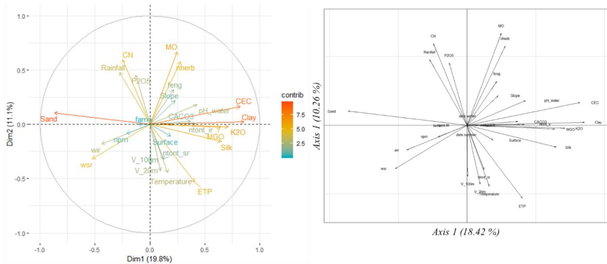
Figure 12: Correlation circle of environmental variables with their contribution on the left and with the habitat and the sampling period on the right
