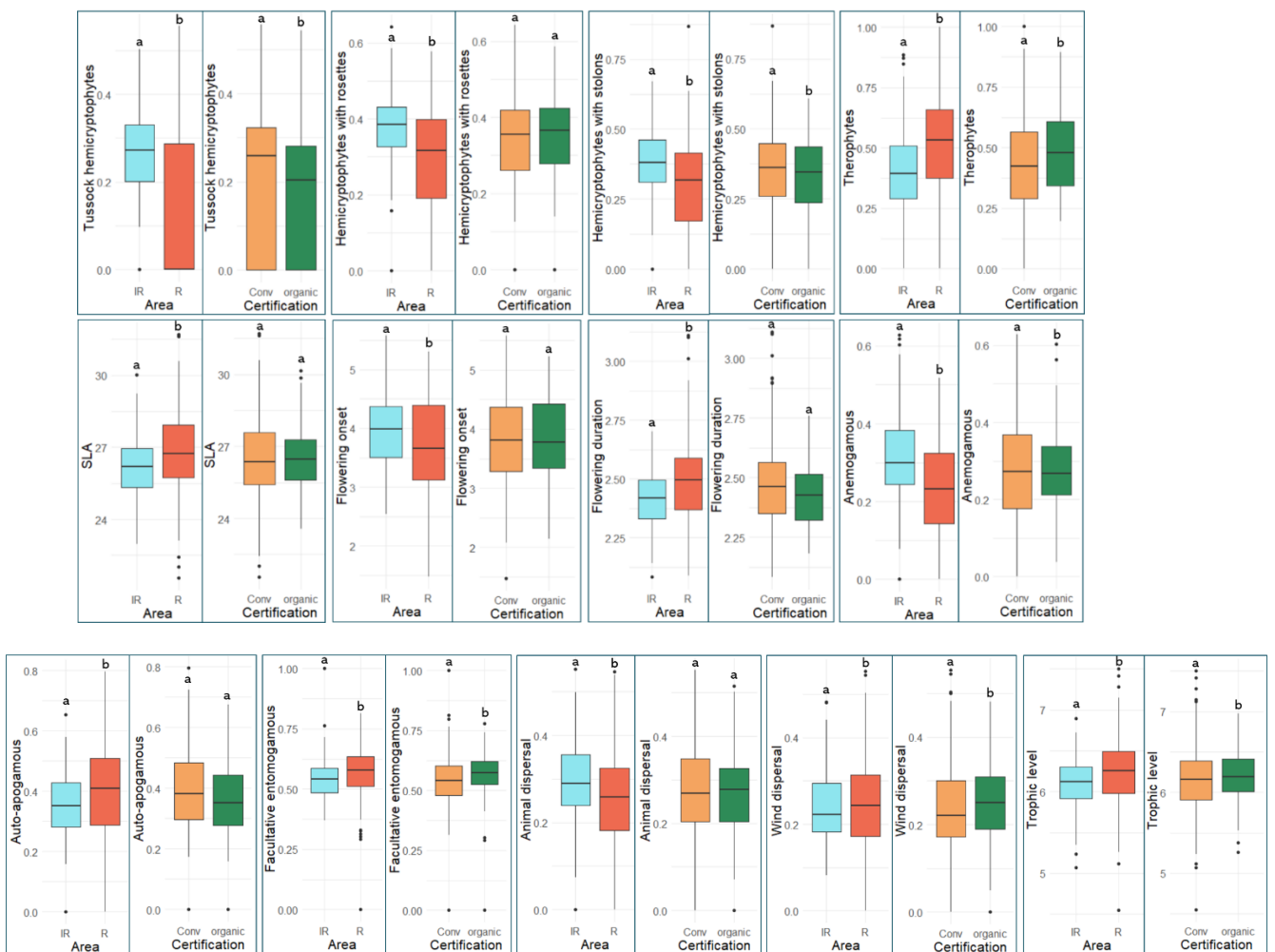
Figure 13: Boxplots of CWV of traits with the areas in blue for the inter-rows, in red for the rows, in yellow for conventional and in green for organic production mode.
