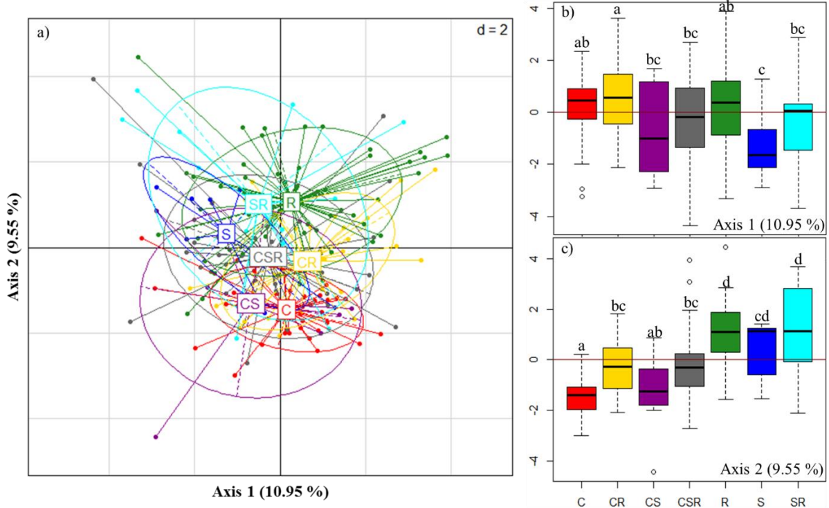
Figure 4: Grime strategies as supplementary variables on the Hill & Smith analysis (a), C: Competitor, S: Stress-tolerant and R: Ruderal, and the significance of the distribution along the 1 st axis (b) and the 2 nd axis (c) of the multivariate analysis
