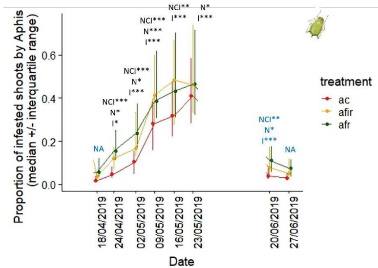
Figure 13: Evolution of the proportion of infested shoots by Aphis sp per tree (median and interquartile range by treatment). Figure and analysis were made excluding not infested trees. Results of significance using GLMM date per date are provided ( n=45 trees). In blue: all the date with a median less than 5% of infested shoots are hardly interpretable. Monitoring had to be stopped between May 27 th and June 17 th . ac: Agricultural control; afir: Agroforestry Inter-row; afr: Agroforestry row. NA: date for which there were not enough observations to run the model. NCI: NCI effect; N: More infested shoots on the North side (Azimuth effect); I: Inflorescence more infested (Shoot type effect). NS: Not Significant; *: <0.05 ; **: <0.01 ; ***: <0.001
