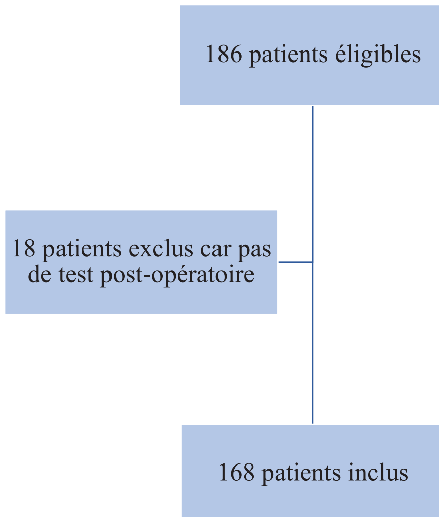
Figure 6 : Flow Chart
