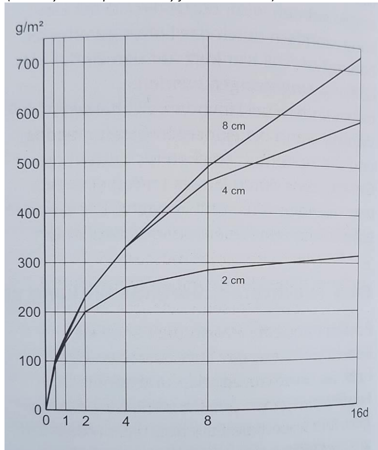
Minke, Diagram 1.4 – 6 Humidity absorption of clay plaster relative to thickness (humidity raised spontaneously from 50% to 80%)
