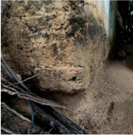
Image 71: Corners; a laterite-stone sits above the earthen base-course (Survey no. 1).
