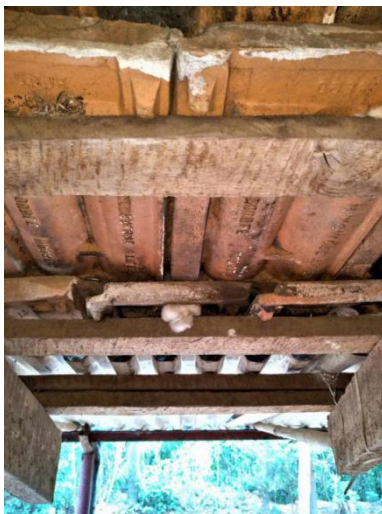
Image 127: Two, instead of one baton was fixed along the ends of the roof's framework (Survey no. 13). Image 128: Splits of the beetle-nut tree were used as batons. Two batons were used along the roof-line. (Survey no. 12).
