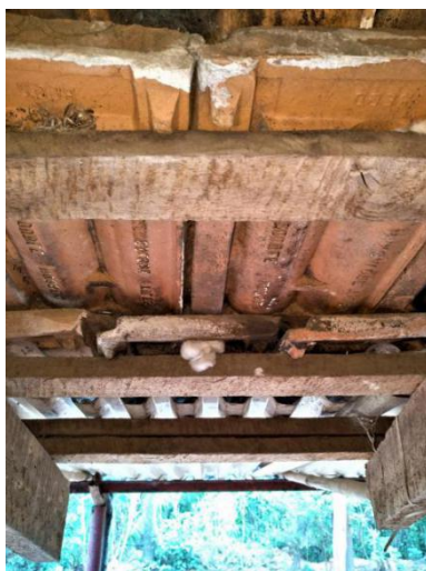
Image 127: Two, instead of one baton was fixed along the ends of the roof's framework (Survey no. 13).
