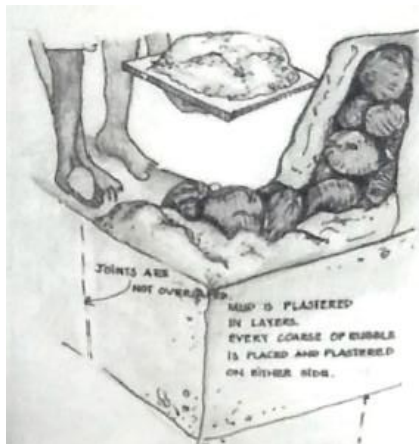
Image 35 and Image 36: Composition of a composite wall.
