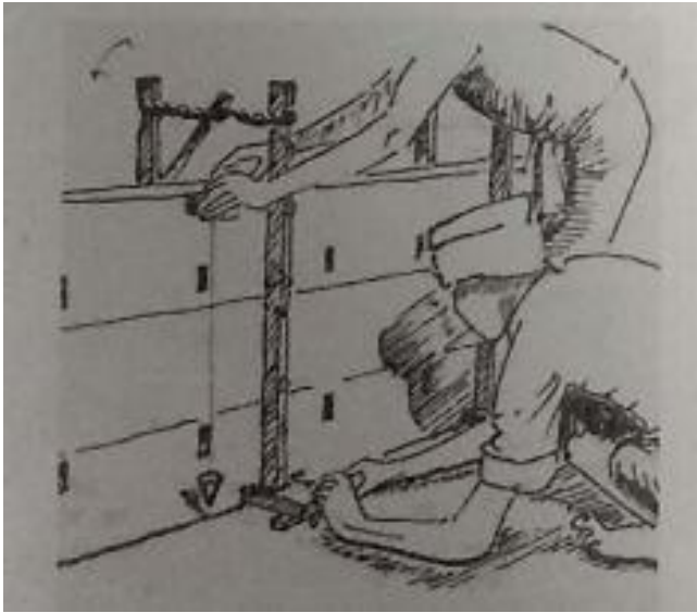
Checking levels with the plumb. [Source: Lobo, Earth in Architecture , p.43]
