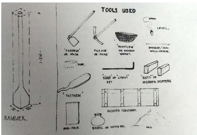
Parts of the form-work with bolts and spacers, and tools [Source: Lobo, Earth in Architecture , p.44]
