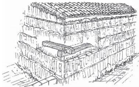
Image 188: L-shaped element at the corners, inside the rammed-earth walls.
