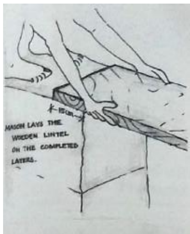
Image 37, Image 38, Image 39, Image 40, Image 41 and Image 42: Construction process, composite walls in Goa.
