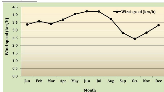
Figure 5: Mean monthly variation of average wind speed from 2002 to 2015.
