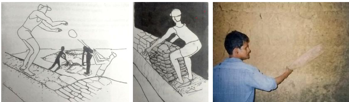
Image 31, Image 32 and Image 33: Cob construction process in Goa.
