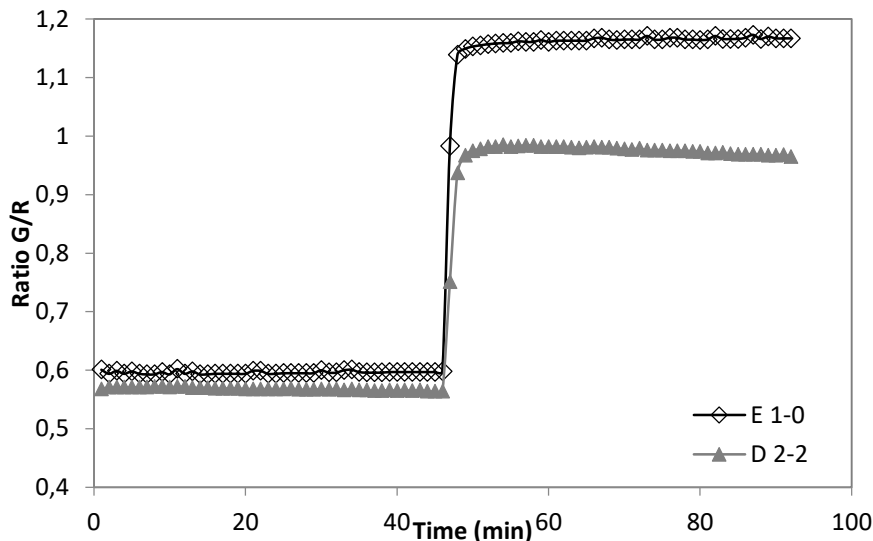
Figure 38: Response time curve of optode E, without titanium oxide.
