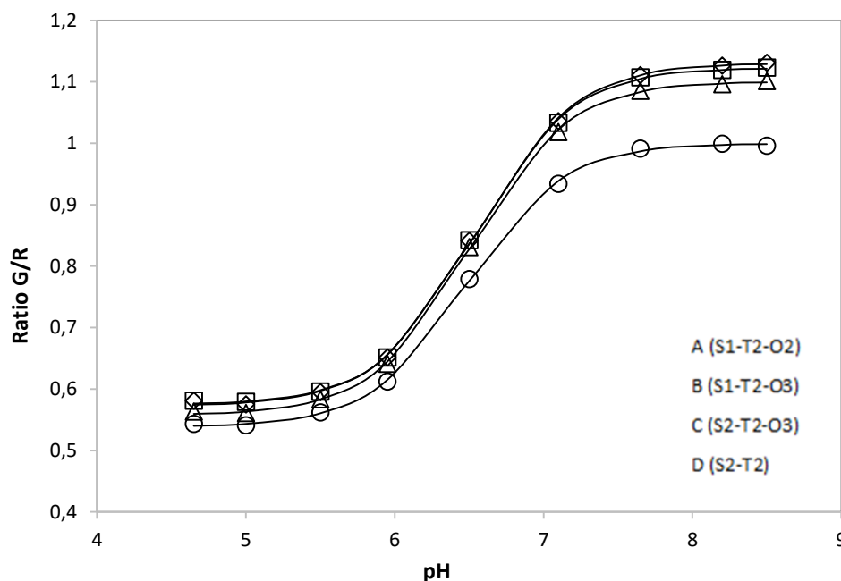
Figure 36: Calibration curve of optode A, B, C, D. Error bars (standard error) are smaller than symbol size. ( n = 150 \times 150 pixels)
