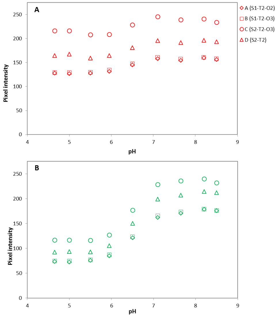
Figure 35: Pixel intensity of Red (A) and Green (B) image of LO optodes at various pH values. SxTxOx represents the thickness of each layer with S for sensor layer, T for titanium oxide layer, O for optical insulation.
