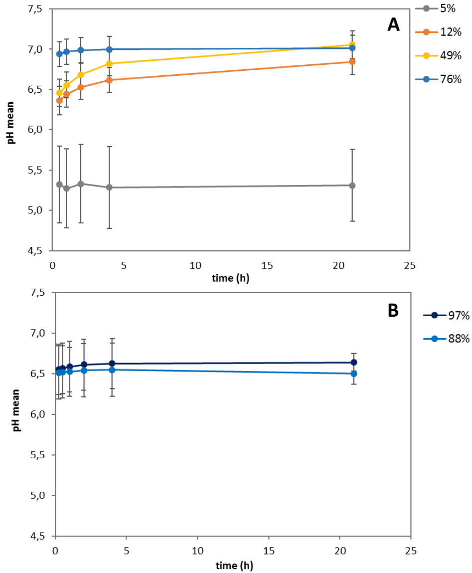
Figure 63: pH changes over time, for each water contact. (mean of 62500 pixels, with SD). (A) Exp I: 5% to 76% of MWHC. (B) Exp II 88% and 97% of MWHC.
