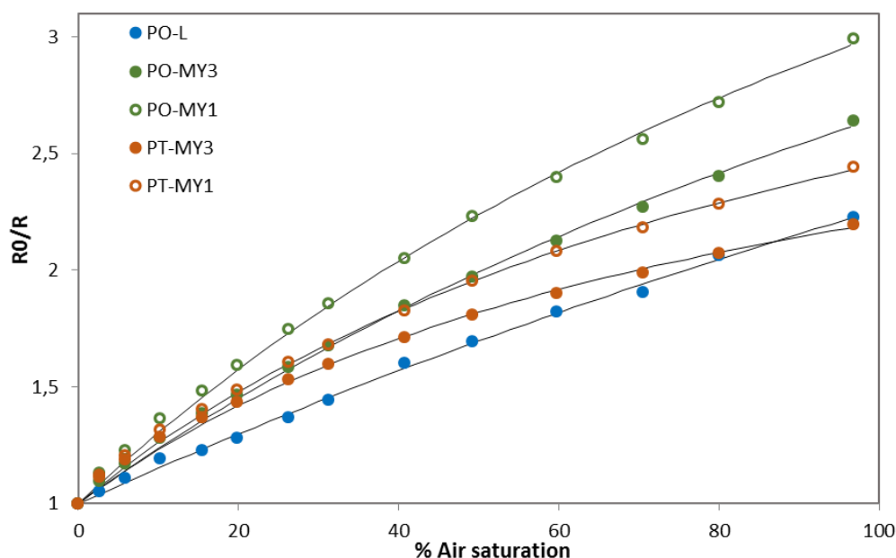
Figure 32: Stern-Volmer plot of of PO-L, PO-MY1, PO-MY3, PT-MY1 and PT-MY3.
