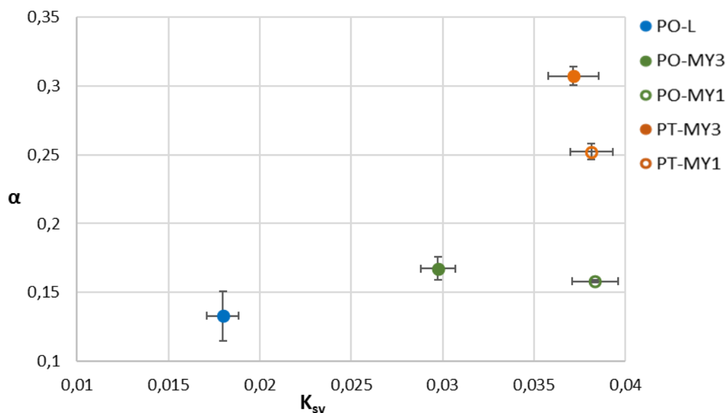
Figure 33: K_{sv} and \alpha parameters estimated from Stern-Volmer model of of PO-L, PO-MY1, PO-MY3, PT-MY1 and PT-MY3.
