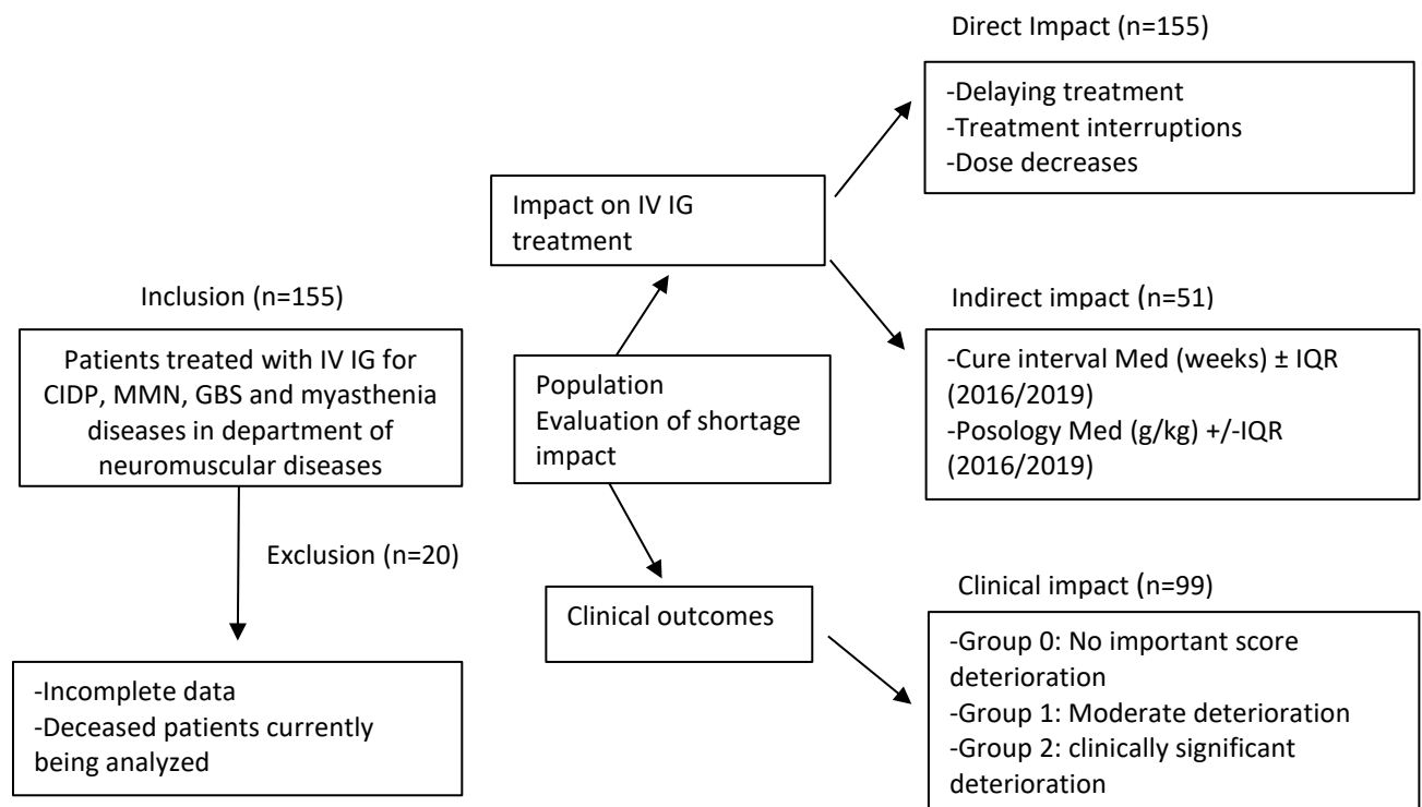
Figure 1 Study design
