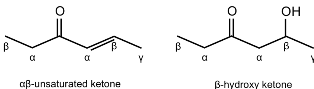
Figure 2 Structure of \alpha\beta -unsaturated ketone and \beta -hydroxy ketone moieties present in withanolides
