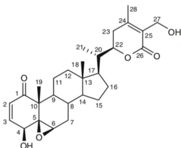
Figure 1 Structure of withaferin A (Misico et al., 2011)
