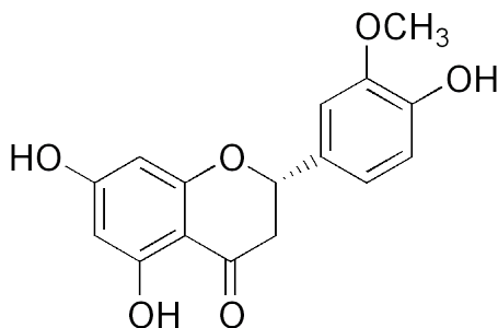
Figure 3 : Homoeriodictyol (PubChem)
