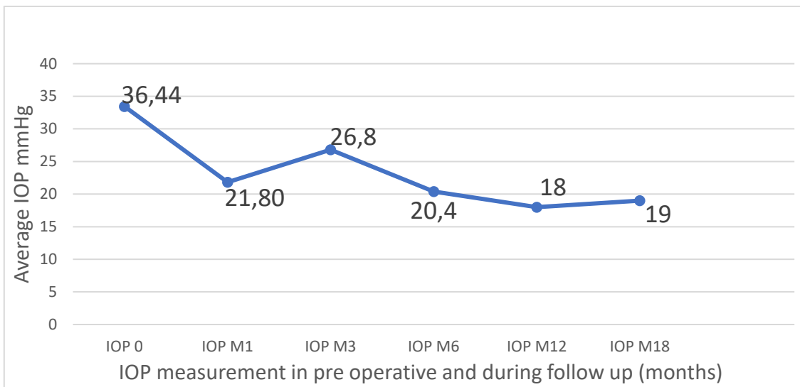
Figure 2 : The average intraocular pressure in pre-operative and during follow-up.
