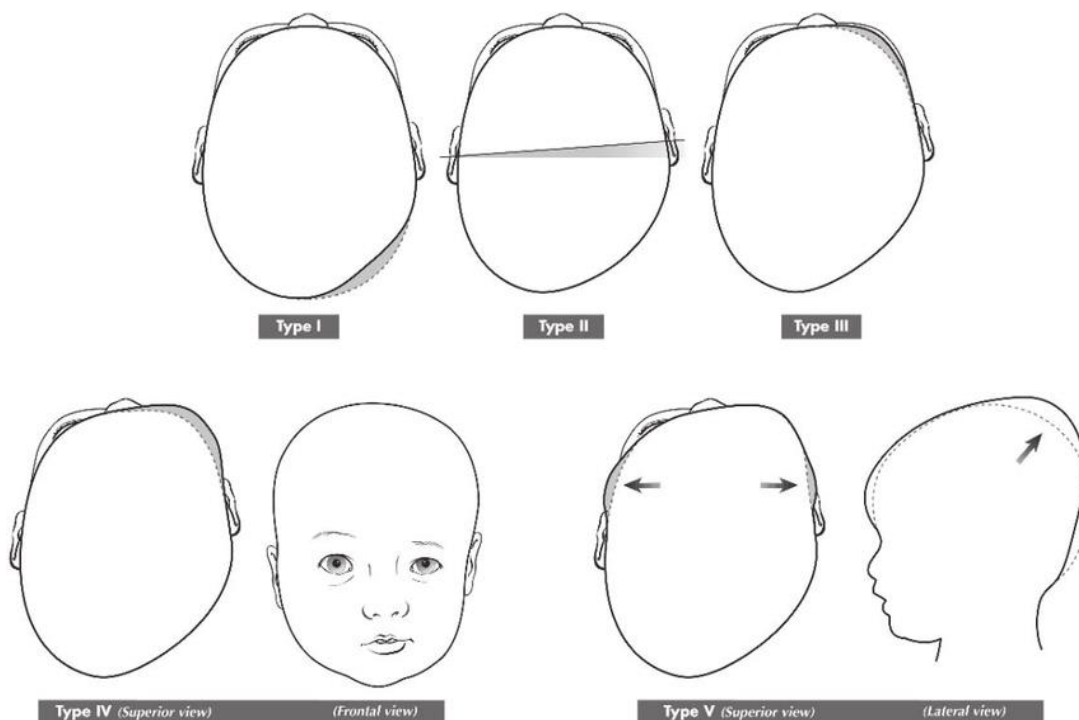
Figure 3 : Classification d'Argenta
