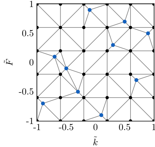
Figure 3.3: Basic mesh configuration (regular grid n^0 ( \bullet ), Latin hypercube nodes n_{LHS} ( \bullet )) and the corresponding Delaunay triangulation (—).
