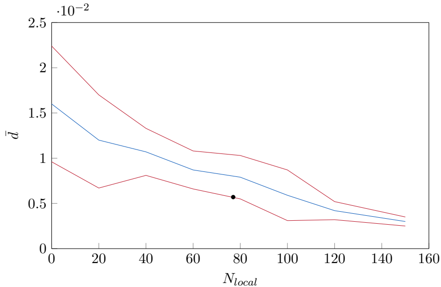
Figure 4.4: Mean variation distance \bar{d} as a function of the number of points added during the local refinement N_{local} .
