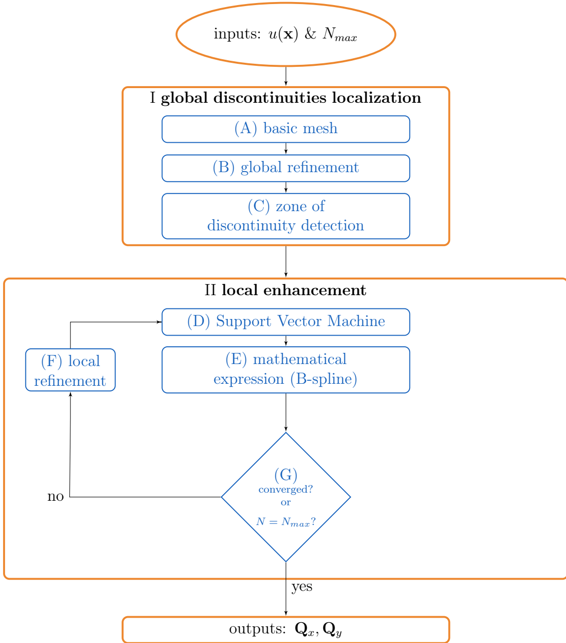
Figure 3.1: Proposed algorithm.
