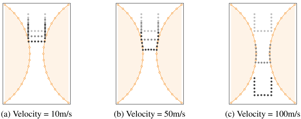
Fig. 4.3 Comparison of different falling velocities for the cube between two rigid rings.
