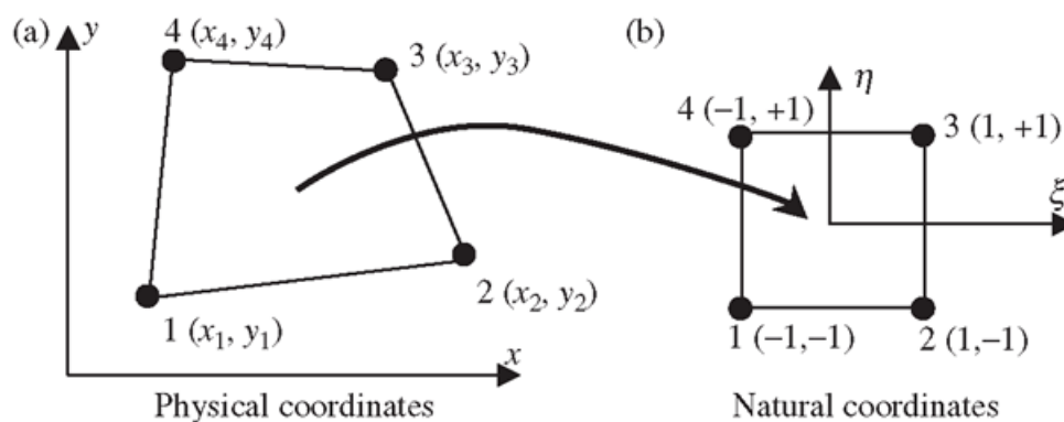
Figure 2.20: Mapping of the physical coordinates of a quadrilateral element into natural coordinates.
