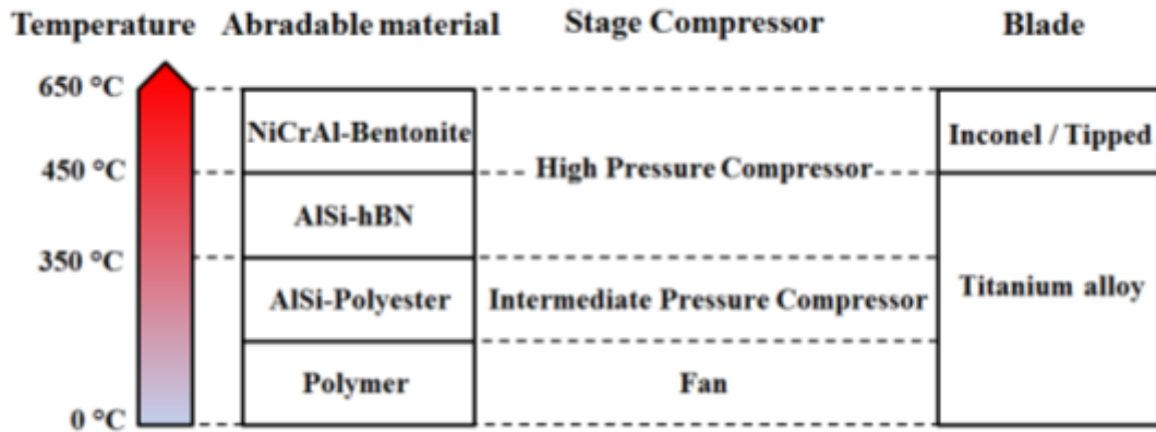
Figure 2.4: Shows the most used abrasible materials in modern engines according to the compressor stage and thus to the environment temperature conditions [3].
