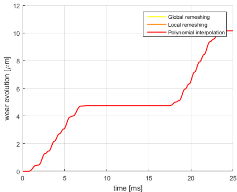
Figure 4.15: Total amount of material worn out from the beam during the evolution of the whole simulation of 25\text{ms} computed using the Penalty method and taking into account the wear evolution by the following three techniques: global remeshing (yellow line), local remeshing (orange line) and polynomial interpolation (red line).
