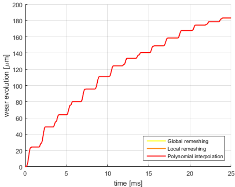
Figure 4.20: Shows, for more severe contact interactions, the total wear during the simulation evolution computed by the Penalty method and taking into account the wear by the following three techniques: global remeshing (yellow line), local remeshing (orange line) and polynomial interpolation (red line).
