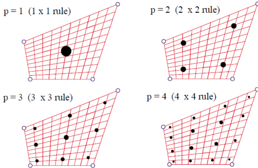
Figure 2.21: Shows the first four product rules for Gauss Integration with equal number of points along the two directions [32].
