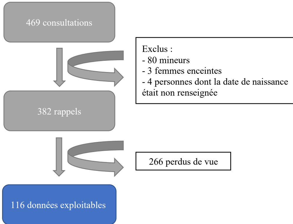
Figure 4: Flow chart
