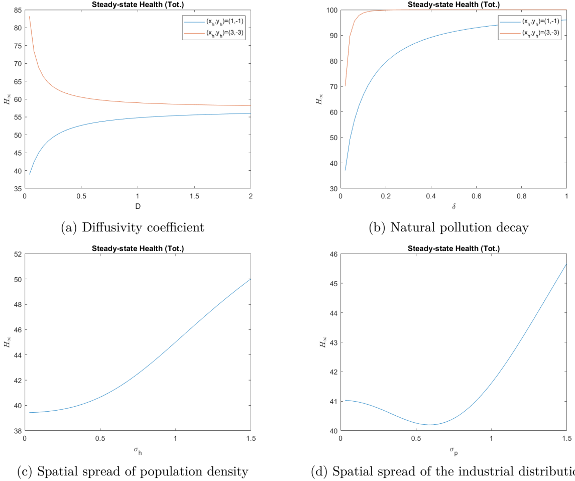
Figure 5: Total health at steady-state as a function of parameter values.
