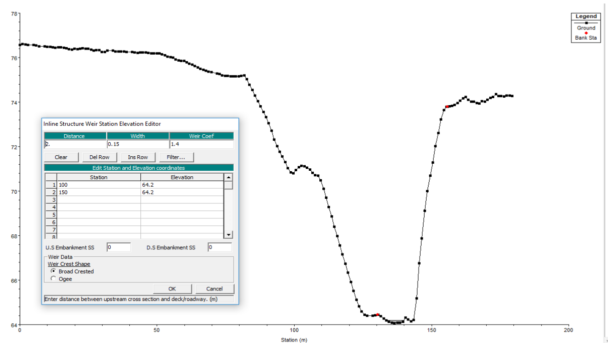
Figure 19 : front view from upstream of the weir, with the characteristics set for it. Balgavies Burn, cross section 320.
