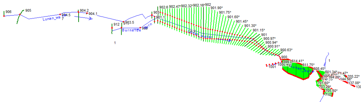
Figure 12 : View of the geometry of one of the models used for the steady state simulation by A. Vinten
