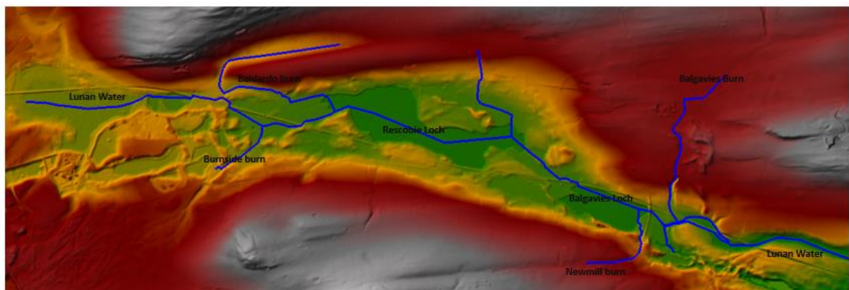
Figure 3 : rivers modelled in the Hec-Ras model of the upstream part of the Lunan Water, similar extend than figure 2
