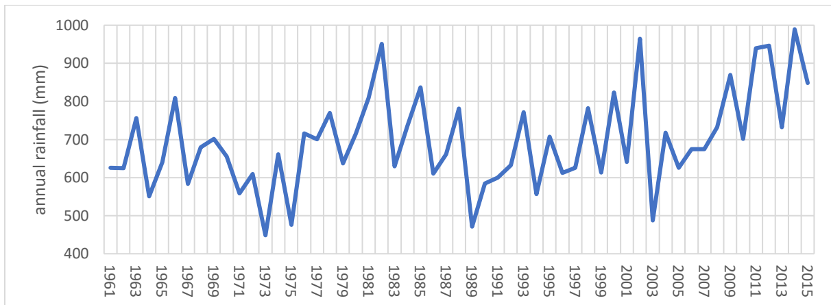
Figure 4 : annual rainfall on the Baldardo Burn catchment, years 1961-2015, data from the UK weather office, data obtained from I. Pohle.
