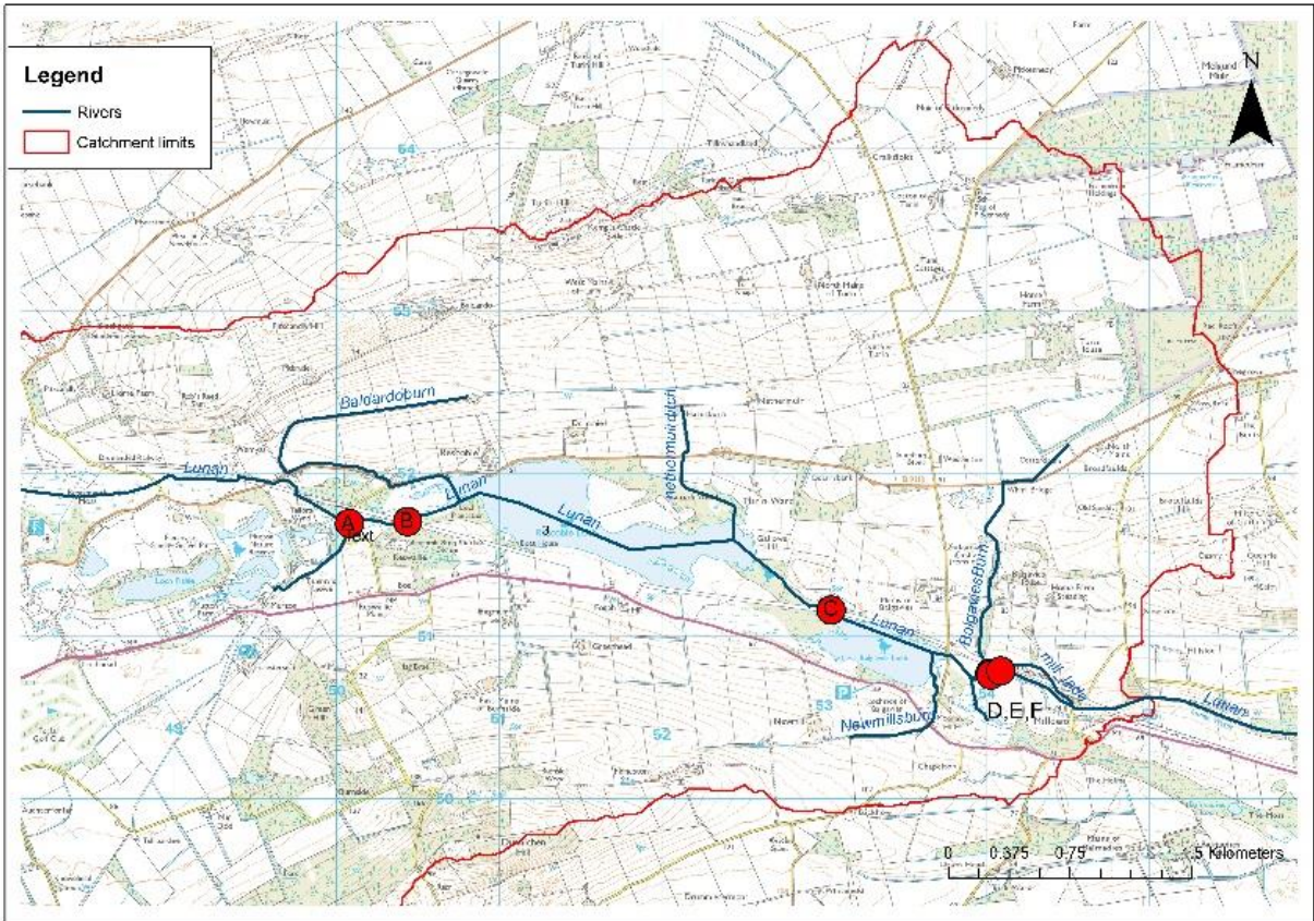
Figure 16 : position of the hydraulic structure modelled in the Hec-Ras model, large scale
