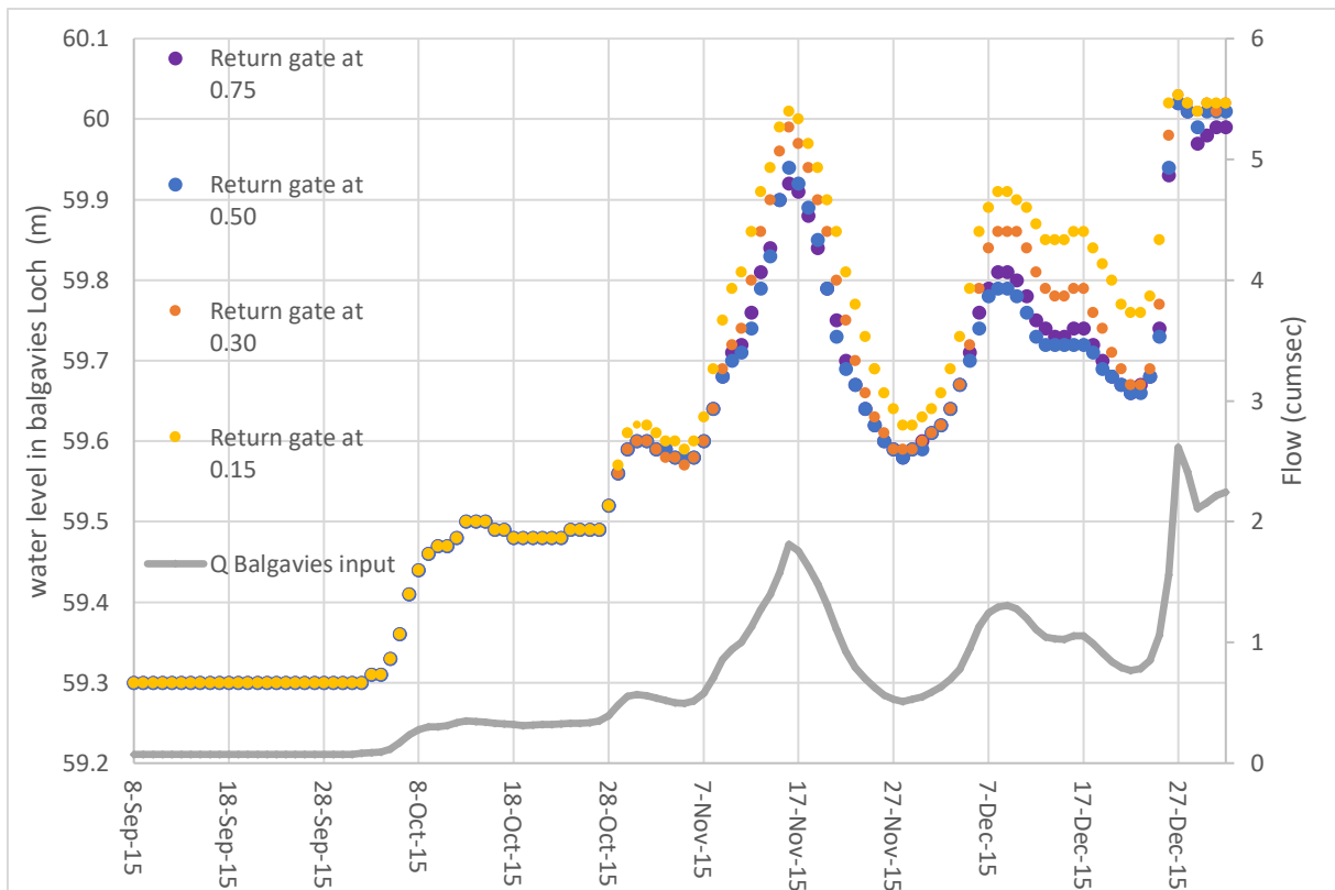
Figure 31 : impact of the different openings in the return gate on the Balgavies Loch level
