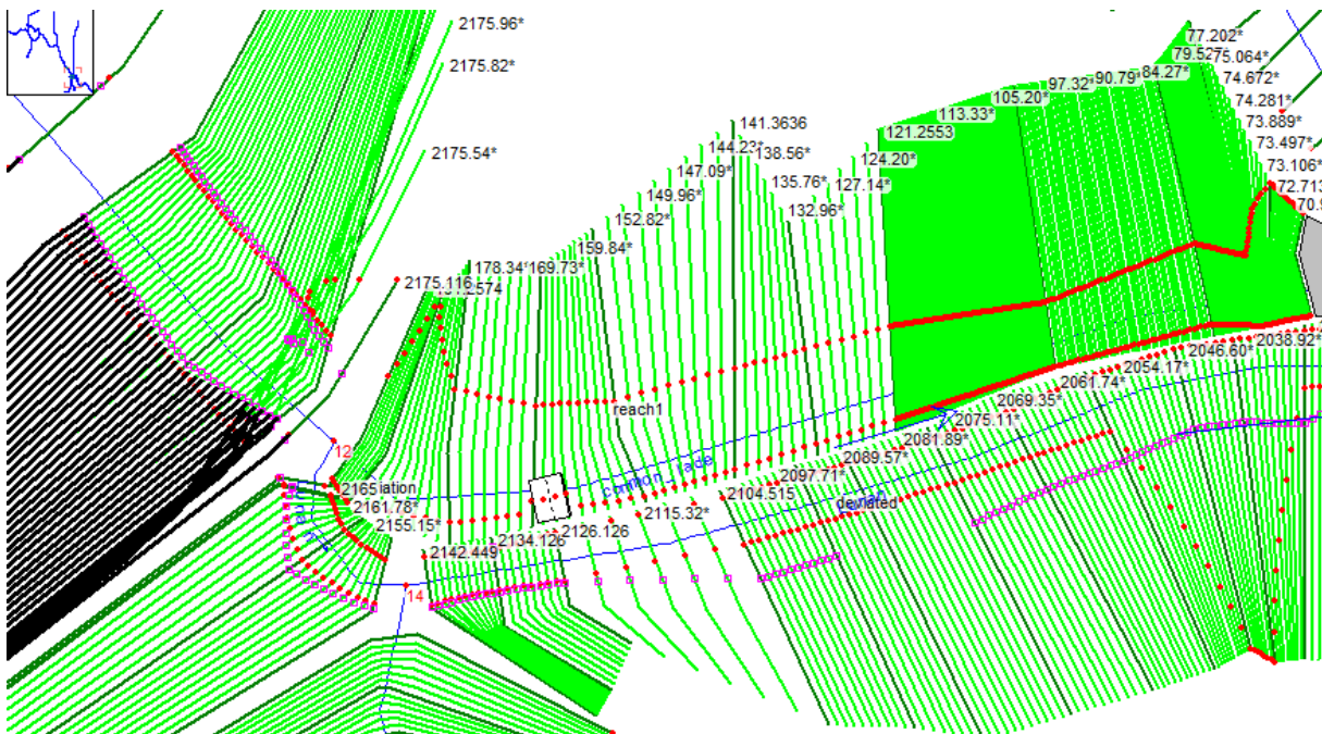
Figure 37 : view of the positioning of the tilting weir, placed on the upstream part of the Common Lade
