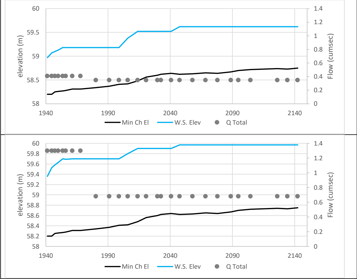
Figure 36 : profiles of the Lunan Deviated channel on the 24 and 29 December with the modified spillway
