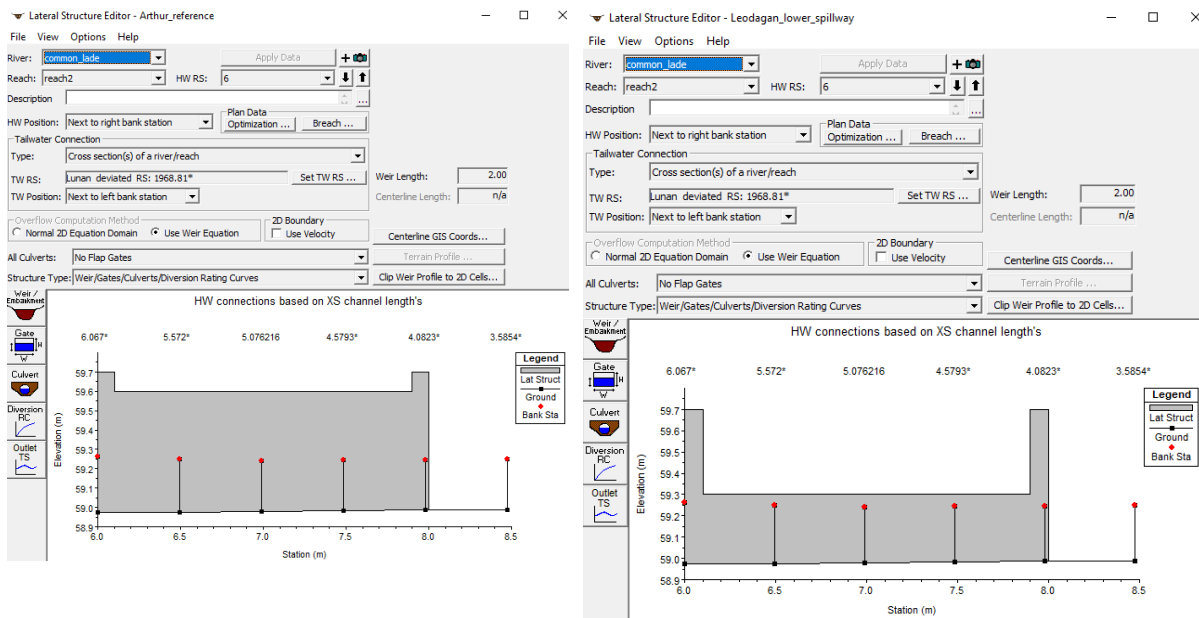
Figure 34 : description of the modification of the lateral spillway in Common Lade
