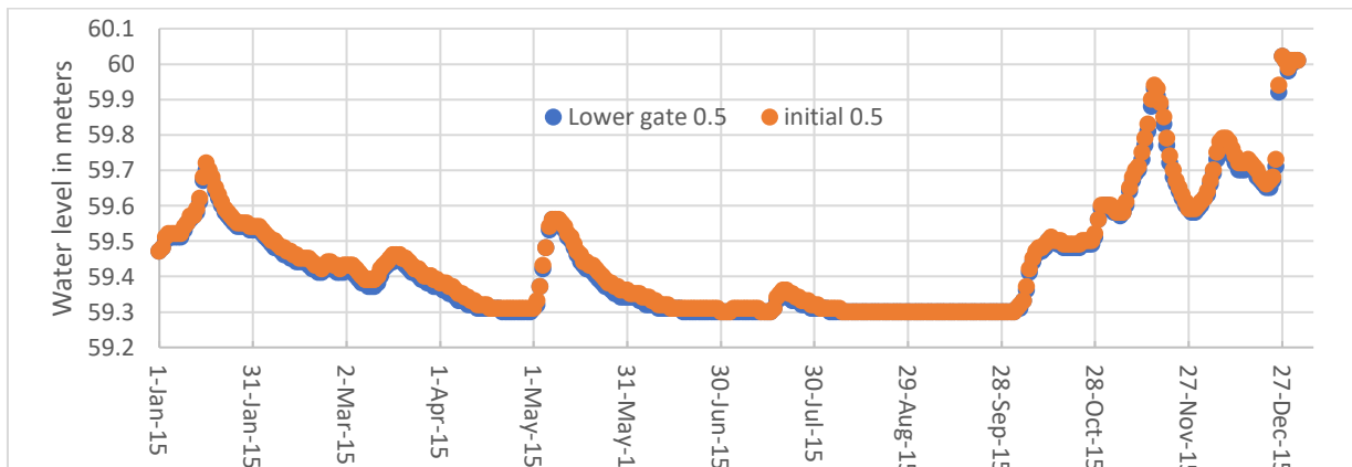
Figure 33 : impact of modifying the return gate inlet in the Balgavies Loch water level
