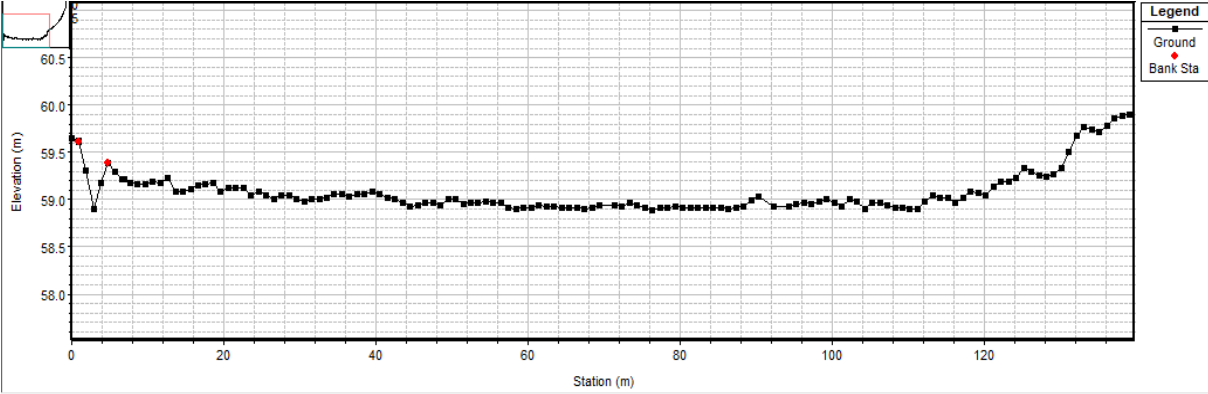
Figure 27 : Lunan Deviated second cross section (3 meters downstream of the spillway), initial geometry
