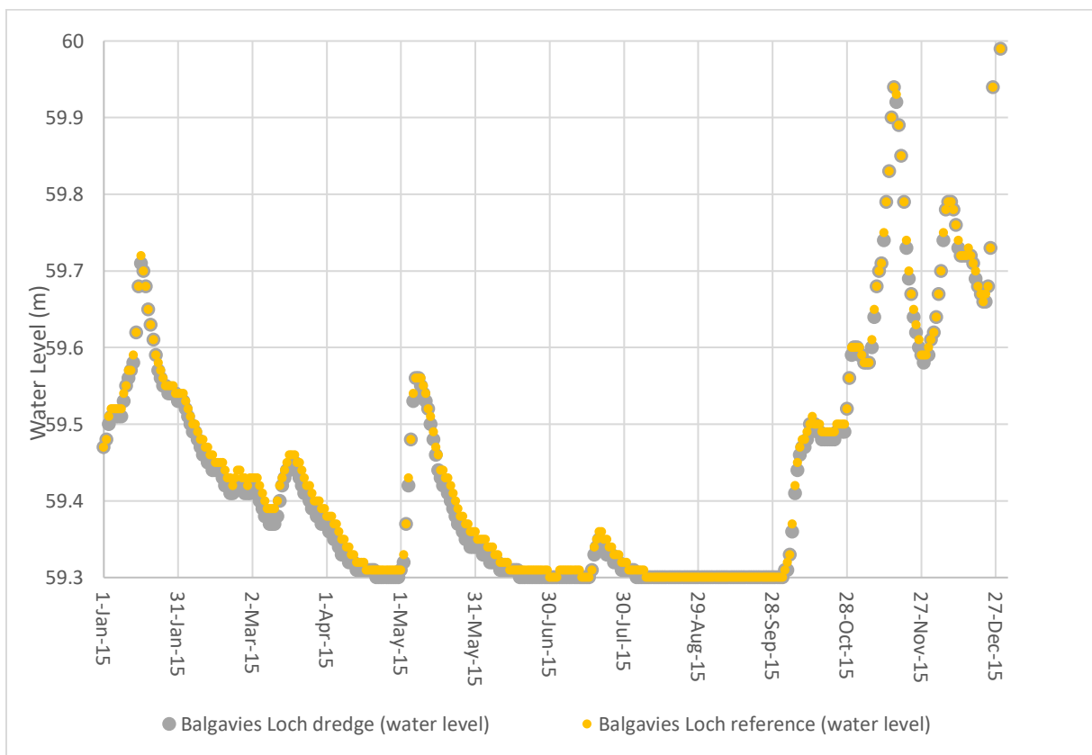
Figure 29 : comparison of water levels from the dredge and reference scenario, with the return gate set with an opening at 0.5 m
