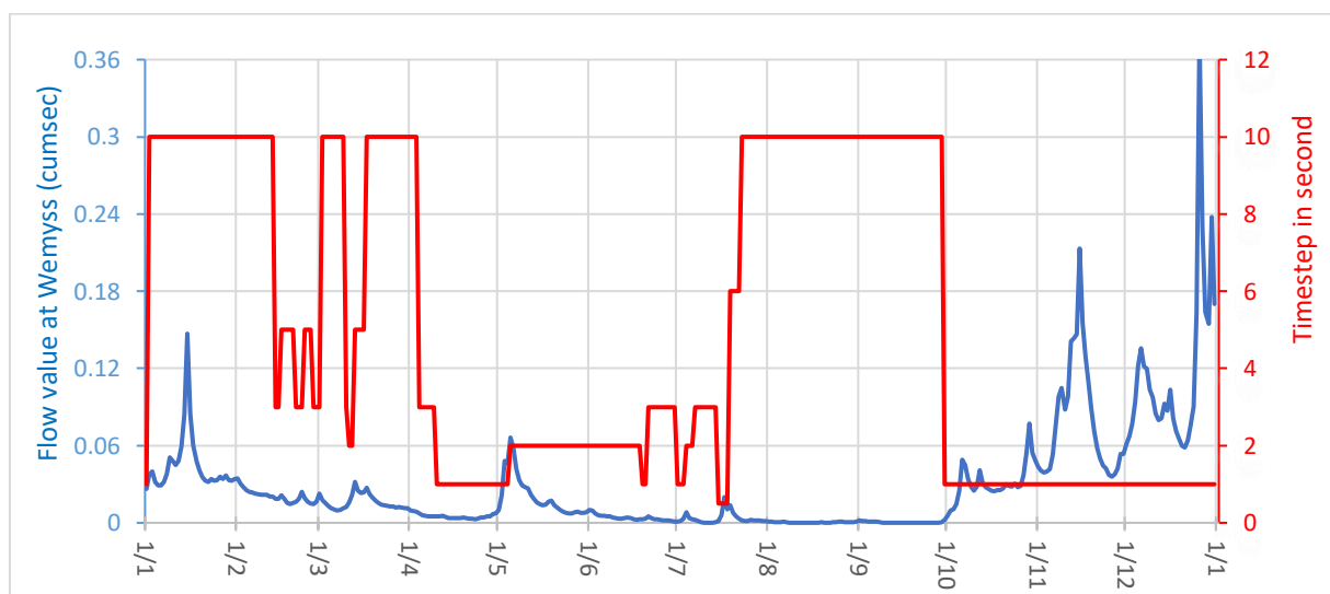
Figure 24 : Plot of the reference flow values and the calculation timesteps used for the simulation of 2015
