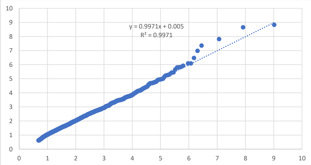
Plot of the initial modified frequency against the frequency calculated with the flow values ( x=f'(Q wemyss), y= modified frequency)
