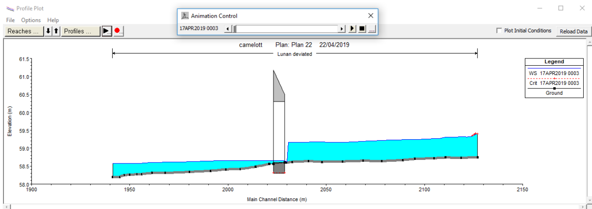
Figure 23 : illustration of initial water level step in the bridge entrance, Lunan channel, bridge labelled “D” on figure 17.
