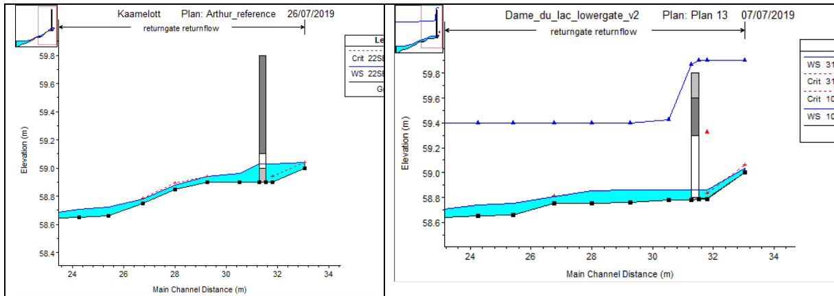
Figure 32 : profile of the return flow channel before and after the gate inlet modification
