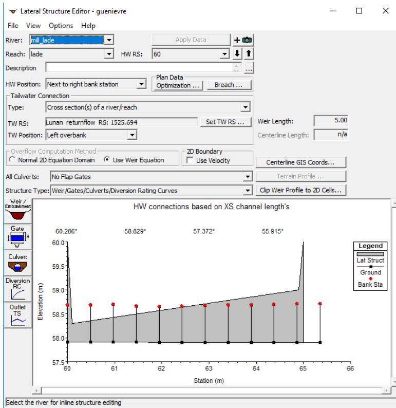
Figure 22 : description of the lateral spillway created in the end of Mill Lade reach
