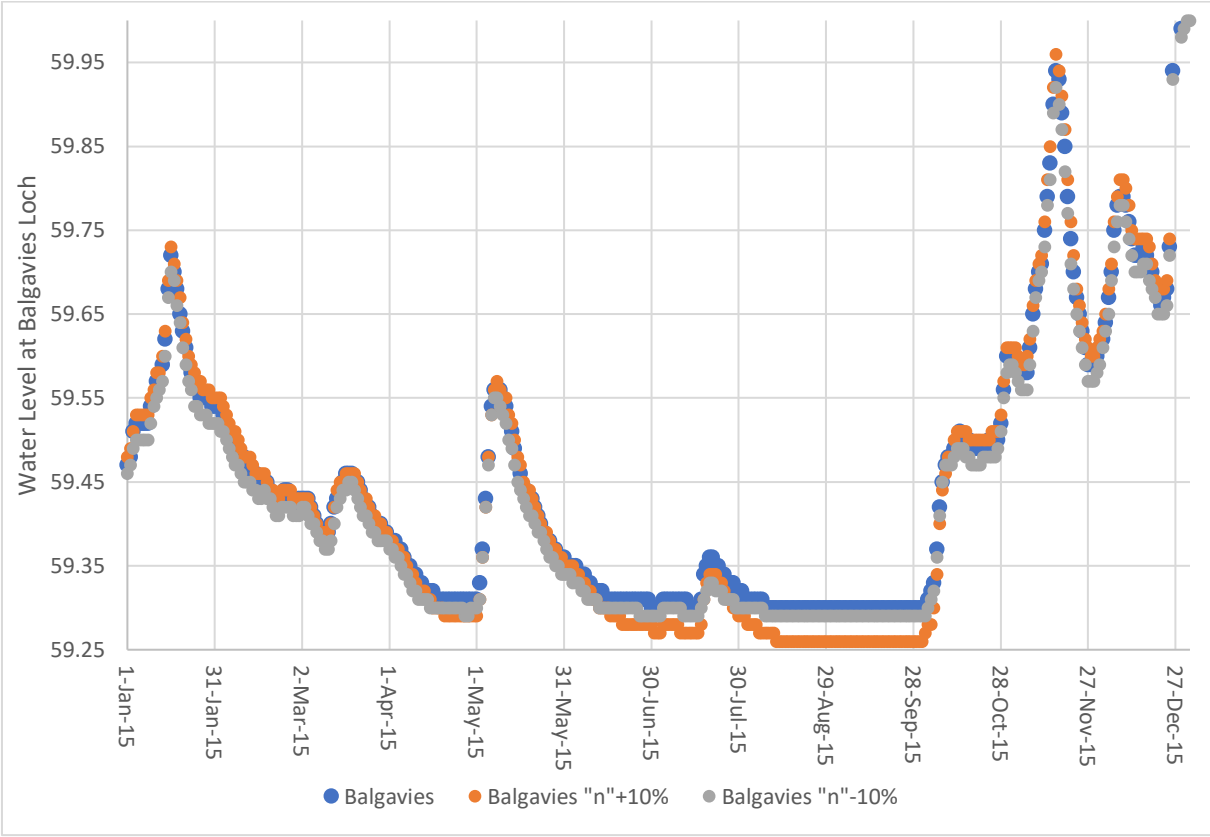
Figure 26 : impact if a modification of the Manning coefficient (n) by ten percent for all the rivers on the Balgavies Loch water level
