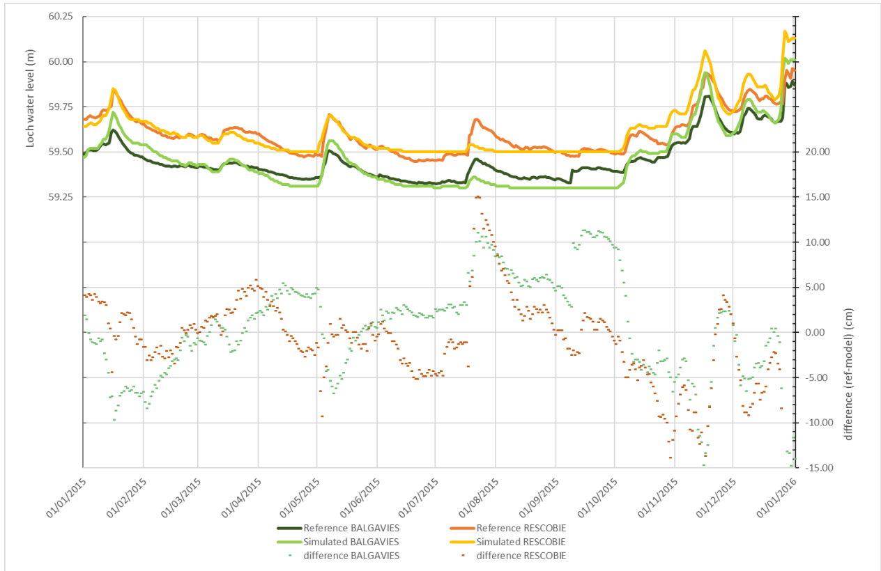
Figure 25 : plot of the measured (reference) and calculated (simulated) water levels in Balgavies and Rescobie Loch in 2015
