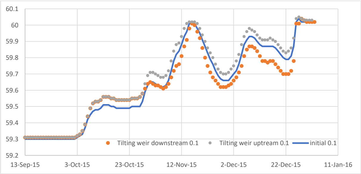
Figure 38 : Water levels in Balgavies Loch for initial geometry and the two scenarios for the tilting weirs
