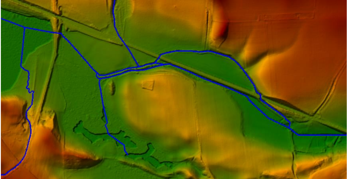
Rivers positioning in the Hec-Ras model, based on field visit and the Compton survey. The river positioning came from the RAS mapper incorporated in the Hec-Ras software.
