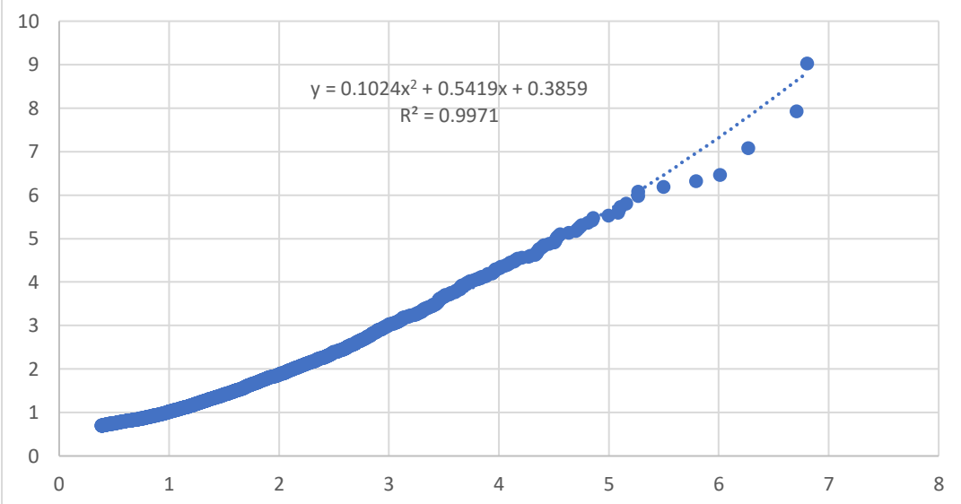
Plot of the function of the flow discovered on the previous plot and the modified frequency ( x=\log function of Q fitted on previous graph, y= modified frequency)
