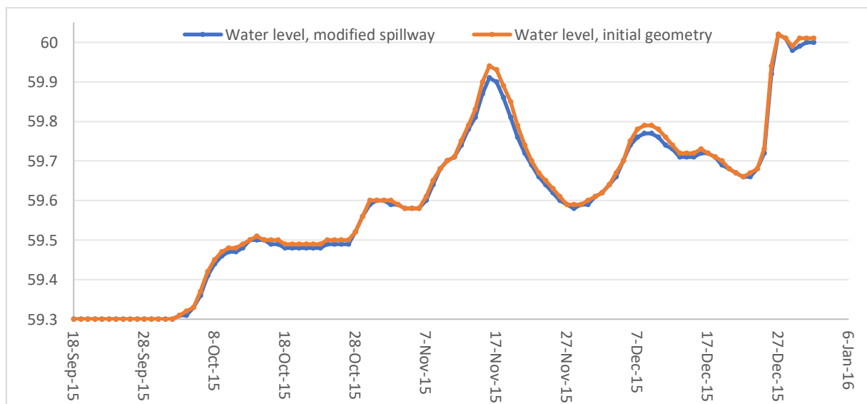
Figure 35 : influence of the modification of the existing spillway on the Balgavies Loch water level
