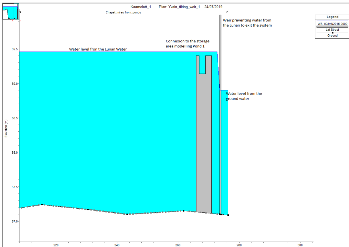
Figure 21 : profile view of the end of the Chapel Mires reach, and the hydraulics structures used to fit the real behaviour.
