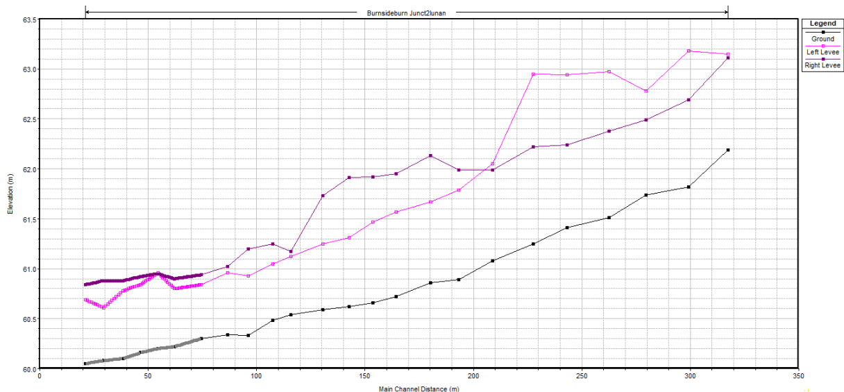
Figure 7 : Profile of the Burnside reach in the Hec-Ras model.
