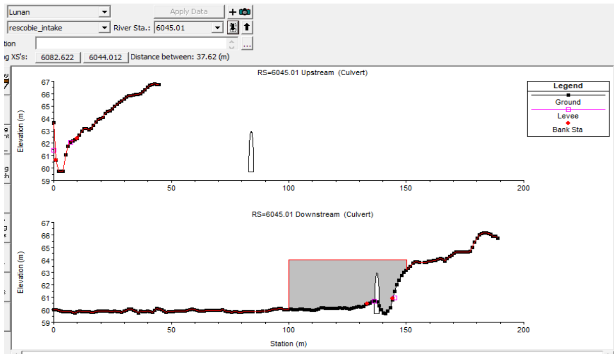
Figure 18 : Inline structure editor view of the rail bridge of Lunan – Rescobie Intake, extracted from the reference geometry
