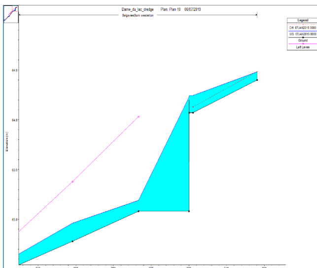
Figure 20 : extract of the profile view for the Balgavies Burn reach, water level calculated for the 7 th Jan 2015 midnight. The x axis is the meters from the junction with "Common Lade"
