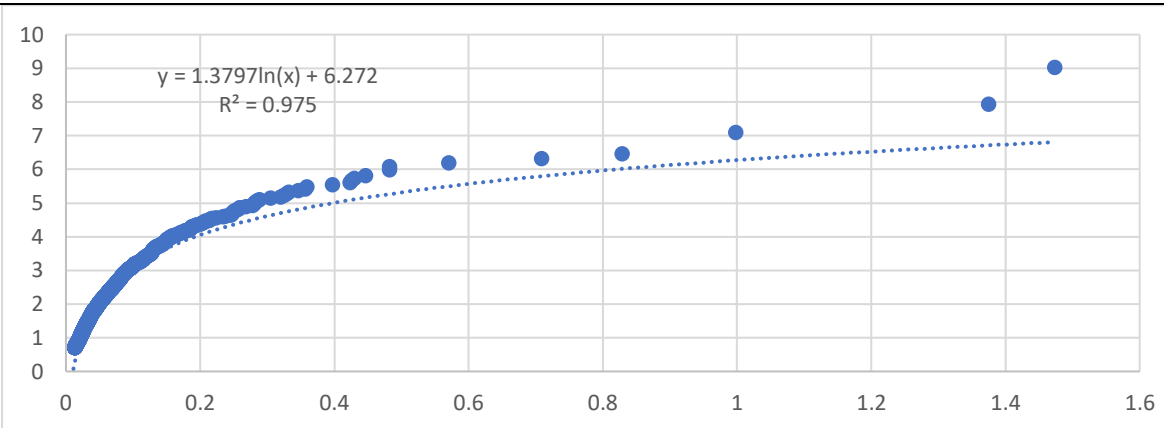
Plot of the modified apparition frequency against the measured flow value ( x=Q at wemyss, y= -\ln(F(Q)) )
