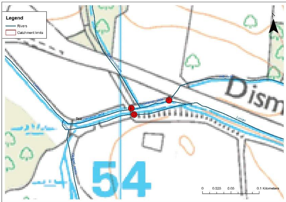
Figure 17 : position of the hydraulic structure modelled in the Hec-Ras model, small scale
