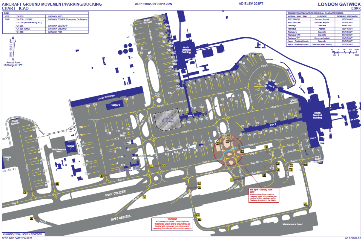
Figure 14 EGKK Aircraft Ground Movement/Parking/Docking Chart Source: (NATS, 2021)
