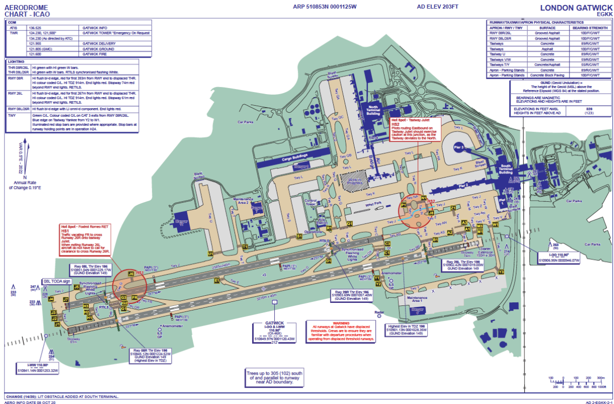
Figure 12 EGKK Aerodrome Chart Source: (NATS, 2021)
