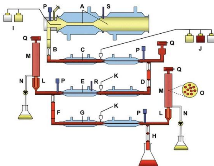
Schematic presentation of TIM-1, equipped with filters to study the bio-accessibility of lipids. A. gastric compartment; B. pyloric sphincter; C. duodenal compartment; D. peristaltic valve; E. jejunal compartment; F. peristaltic valve; G. ileal compartment; H. ileal-cecal valve; I. gastric secretion; J. duodenal secretion; K. bicarbonate secretion; L. pre-filter; M. filtration system; N. filtrate with bio-accessible fraction; O. hollow fiber system (cross section); P. pH electrodes; Q. level sensors; R. temperature sensors; S. pressure sensor
