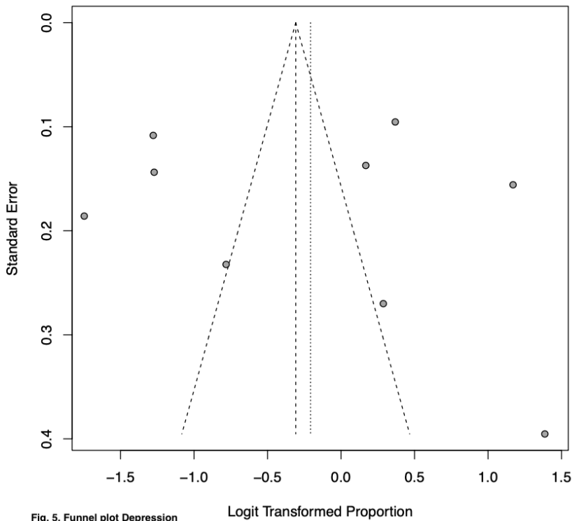
Fig. 5. Funnel plot Depression
