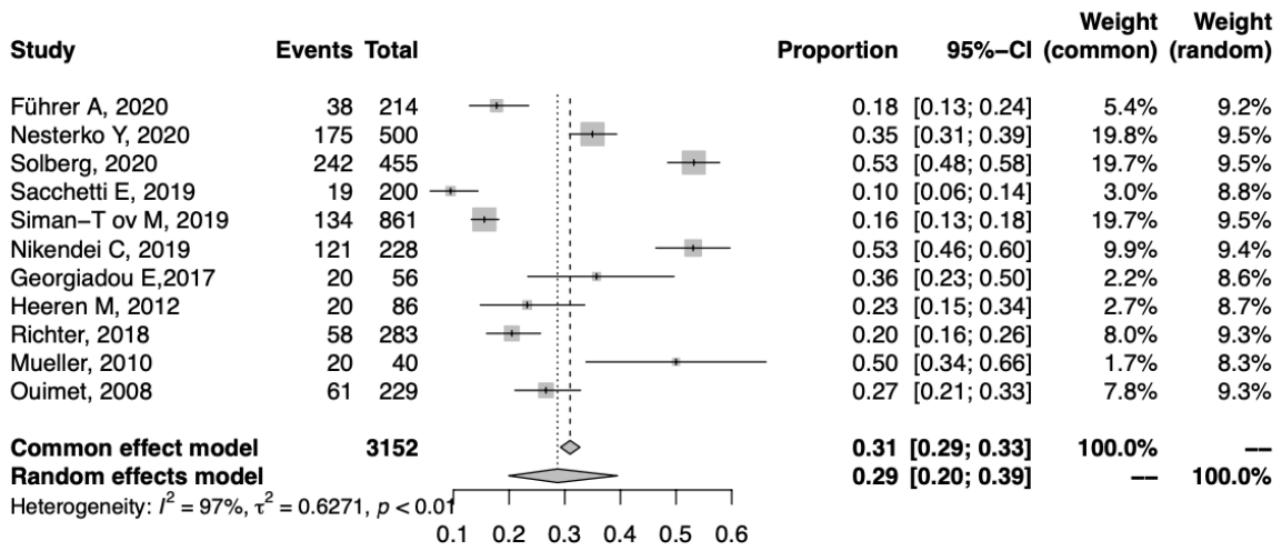
Fig. 2. Forest plot PTSD
