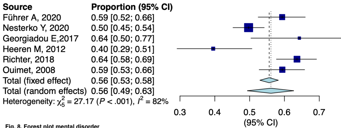
Fig. 8. Forest plot mental disorder
