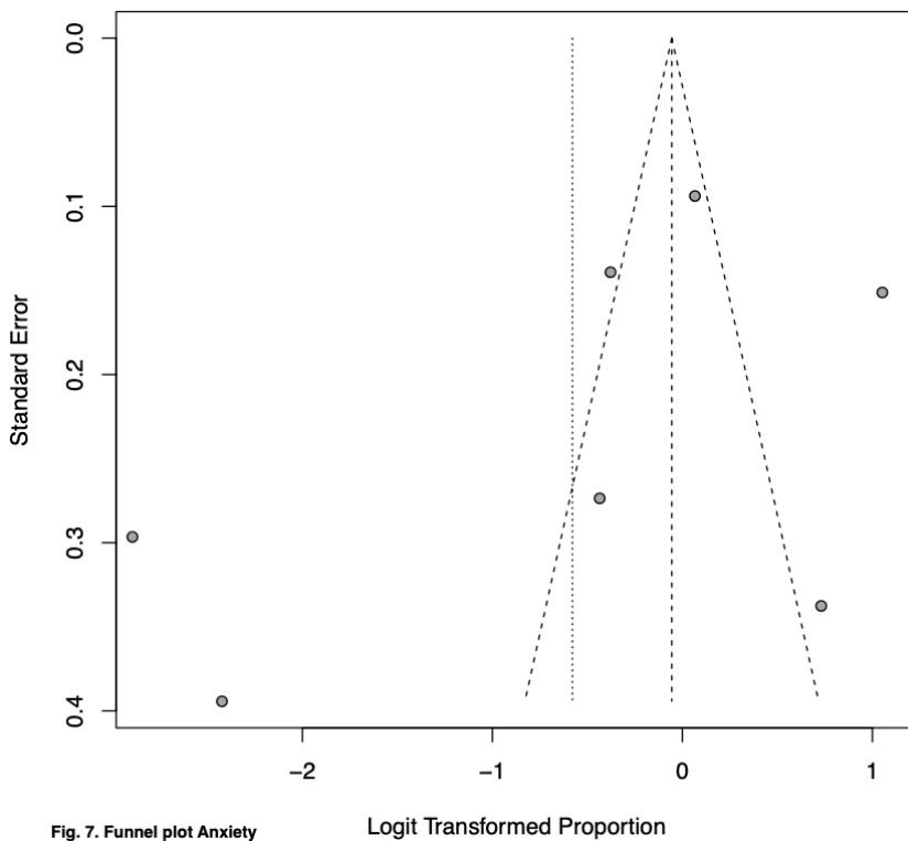
Fig. 7. Funnel plot Anxiety
