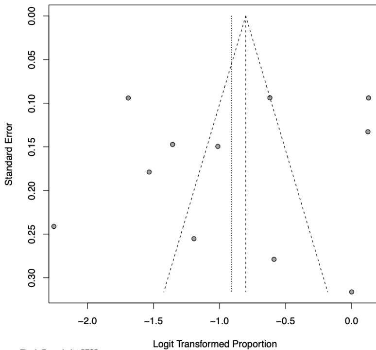
Fig. 3. Funnel plot PTSD
