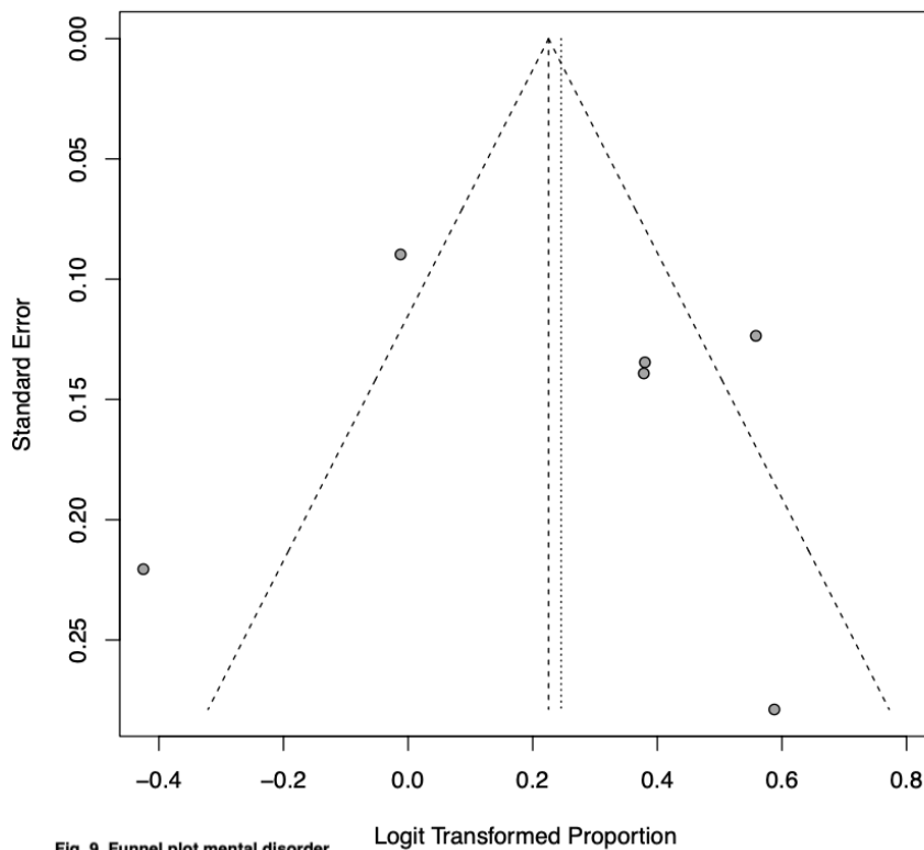
Fig. 9. Funnel plot mental disorder
