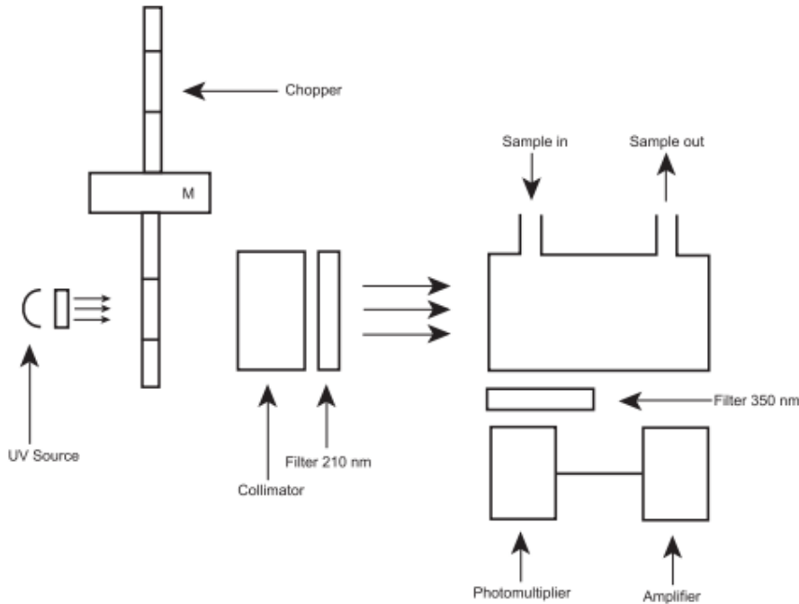
Figure 3098.-1. – UV fluorescence analyser
