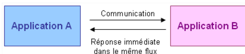
Illustration 9: Communication synchrone.
