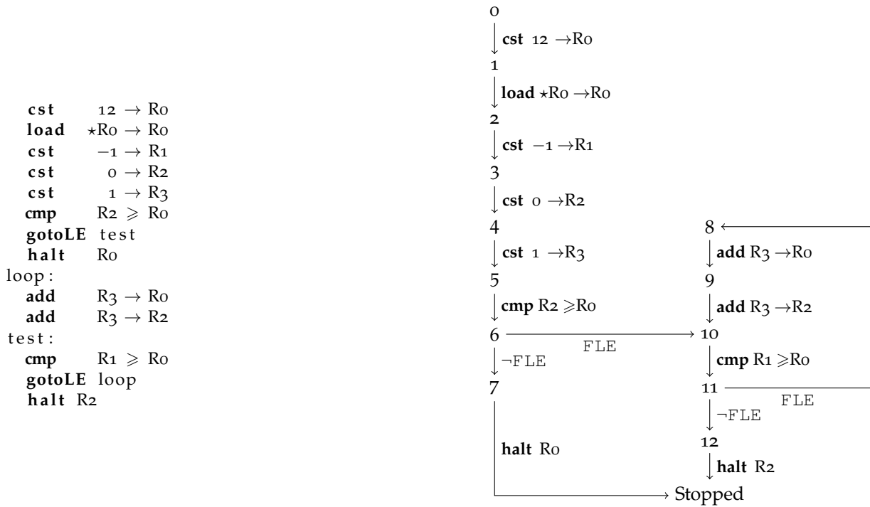
Figure 4.3.: A sample program and its control-flow graph
