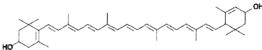
LUTEINE
