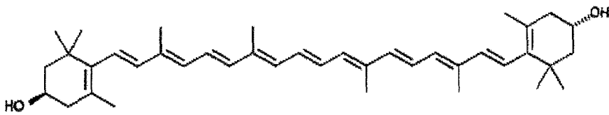
ZEAXANTHINE
