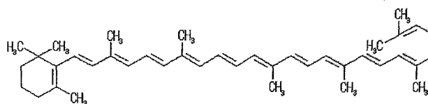
\gamma -CAROTENE
