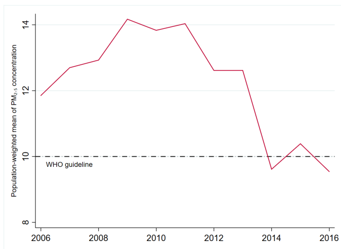
Figure 6: Evolution of average exposure to \text{PM}_{2.5} – 2006-2016
