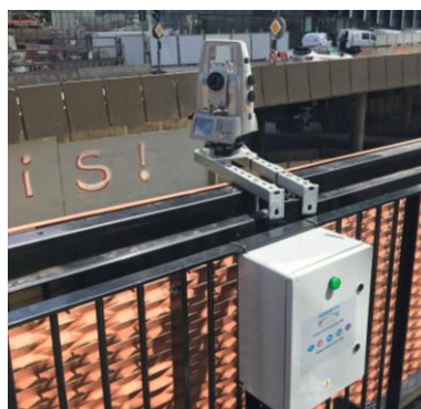
Figure 10: Station totale robotisée (Source : Cementys)
