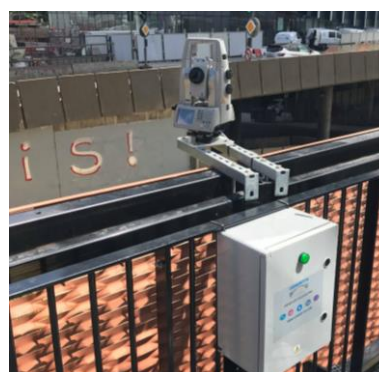
Figure 10: Station totale robotisée (Source : Cementys)
