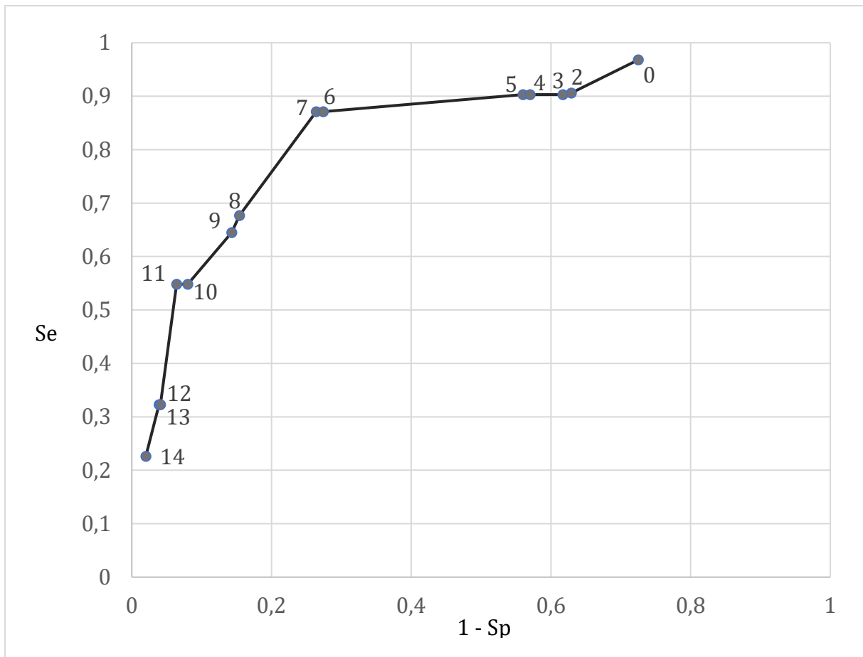
Figure 2. Courbe ROC
